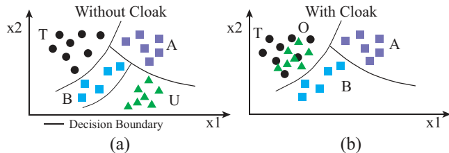
Figure 2: The intuition for why a tracker's model trained on U 's cloaked photos will misclassify U 's original photos, visualized on a simplified 2D feature space with four user classes A, B, U (aka Alice), T . (a) decision boundaries of the model trained on U 's uncloaked photos. (b) decision boundaries when trained on U 's cloaked photos (with target T ).
