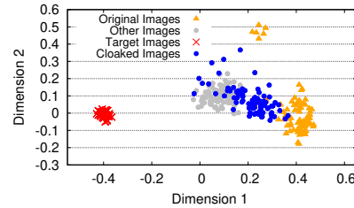
Figure 7: Cloaking is less effective when users and trackers use different feature extractors. (User: VGG2-Dense, Tracker: Web-Incept)
