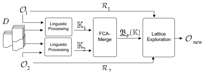
Figure 1: Ontology Merging Method
