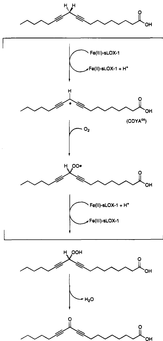
FIGURE 8: Proposed reaction scheme for the formation of 11-oxo-ODYA from ODYA and O 2 , catalyzed by Fe(III)-lipoxygenase. Fe(II)- and Fe(III)-sLOX-1 are Fe(II)- and Fe(III)-soybean lipoxygenase-1, respectively.
