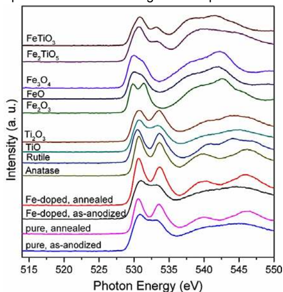
FIG. 6 The O K -edge NEXAFS spectra of pure and Fe-incorporated TiO 2 nanotubes in the as-synthesized and annealed states, compared to those of the oxide reference compounds, showing a negligible difference in the peak features of pure nanotubes upon Fe incorporation.
