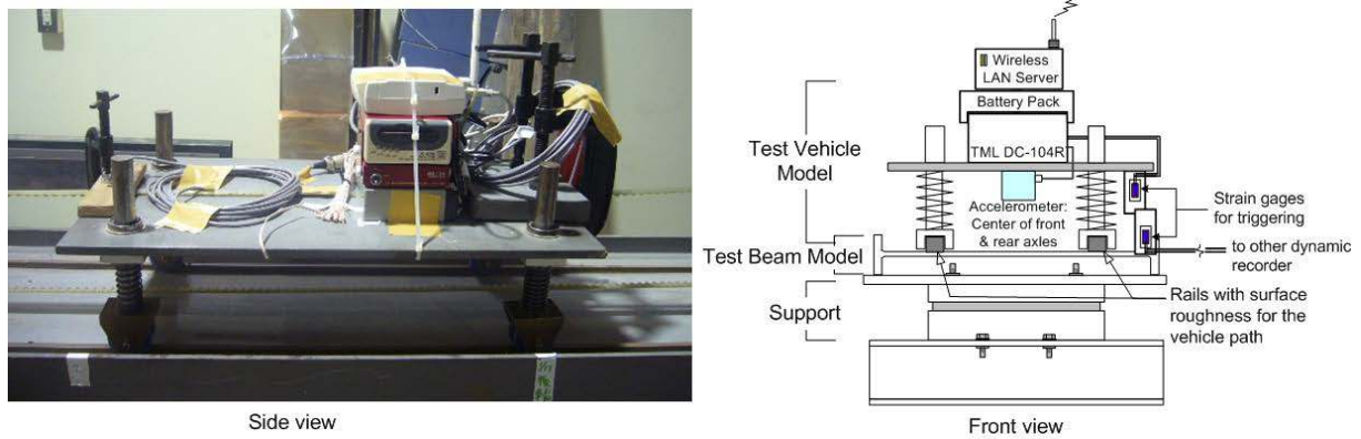
Figure 4. Experimental vehicle.
