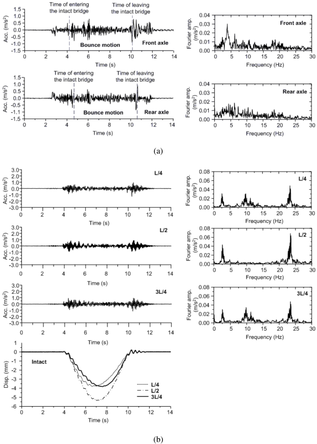
Figure 5. Dynamic responses of intact bridge and vehicle under loading scenario 1 (SCN1): (a) acceleration responses of vehicle; (b) acceleration and displacement responses of girder.
