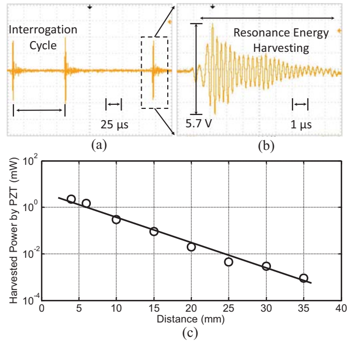
Fig. 4. Measured results showing energy that can be delivered to the transducer using a diagnostic ultrasound: (a) Interrogation pulses measured at the transducer with a load of 10\text{M}\Omega ; (b) Shape of the interrogation pulse showing a resonant response at 3.5MHz; (c) Measured average power levels that can be delivered to the transducer embedded inside PDMS of different thicknesses.
