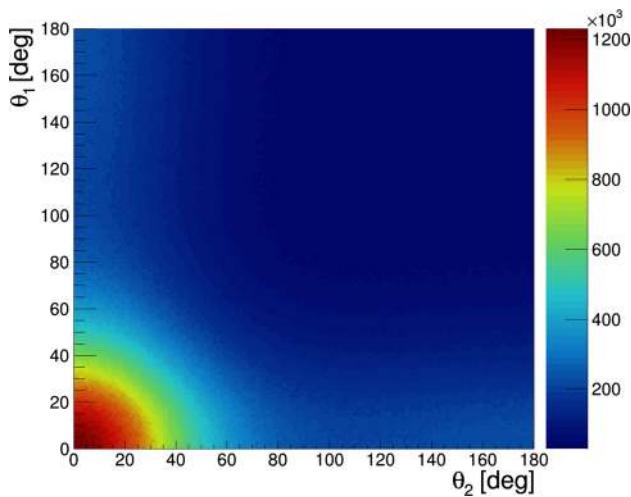
Fig. 11 Event distribution as a function of Compton scatterings angles \theta_1 and \theta_2 simulated for the case of an ideal detector with 100% registration efficiency. The figure is based on 5.96 \times 10^9 simulated events
