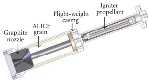
FIGURE 8: Schematic of the flight-weight motor casing.
