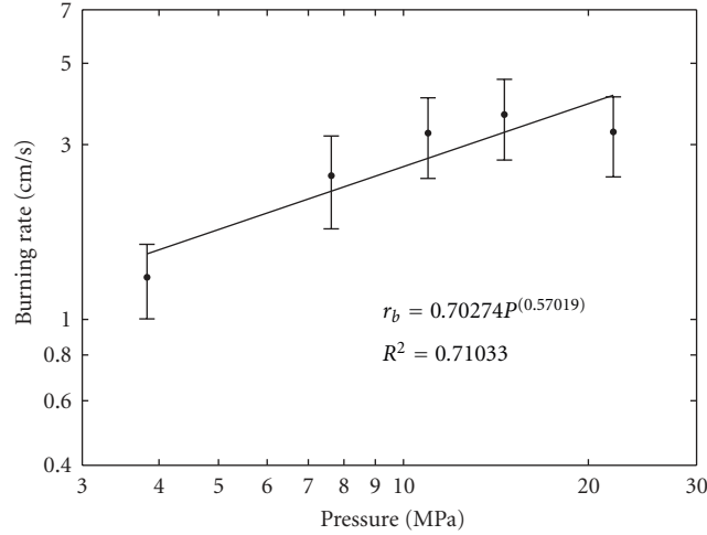
FIGURE 3: Burning rate data of ALICE propellant mixed with the Resodyn mixer.
