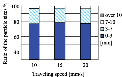
Fig. 28. Comparison for the traveling speeds.
