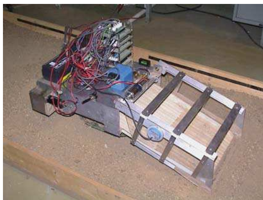
Fig. 14. Excavation type mine removal robot.
