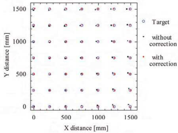
Fig. 13. Result of the position measurement.
