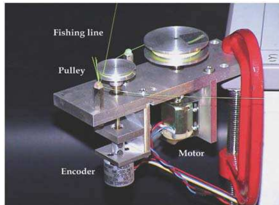
Fig. 12. Positioning sensor unit.
