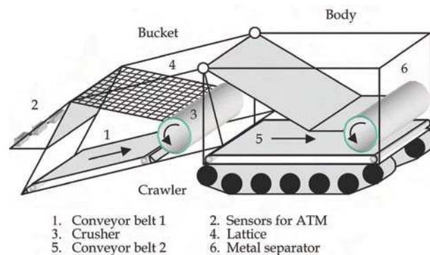
Fig. 2. Conceptual design of the robot.
