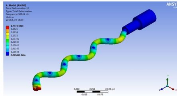
(f) Vibration mode at the frequency of 305.14Hz
