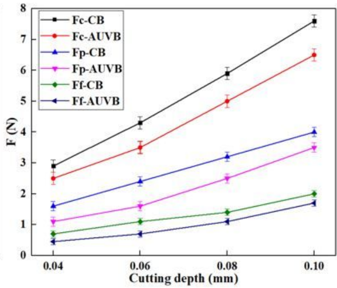
(b) Boring force versus cutting depth
