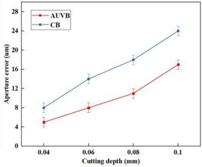
(b) Aperture error versus cutting depth
