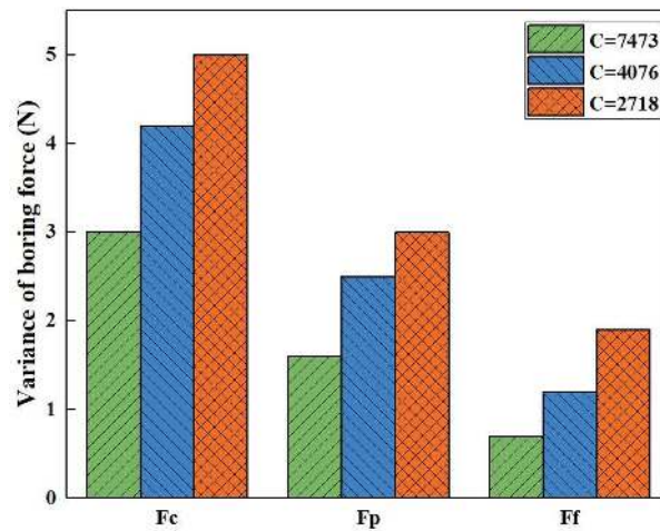
Fig. 14 Influence of size coefficient on boring force for AUVB
