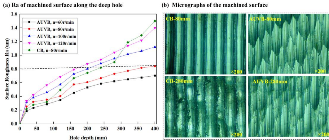
Fig. 21 Roughness (Ra) of machined surface ( D_t=4076 )
