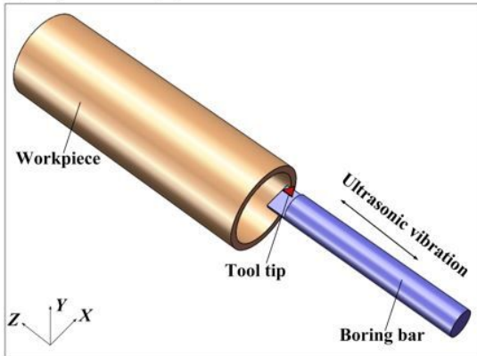
(a) Deep hole boring operation
