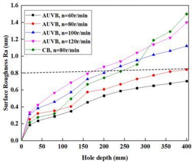
(a) Ra of machined surface along the deep hole
