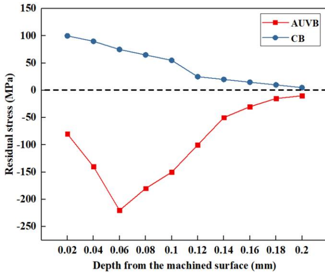
Fig. 25 Residual stress of bored surface ( n=80r/min , a_p=0.1mm , f=0.007mm/r , D_t=4076 )
