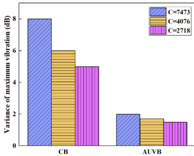
Fig. 20 Influence of size coefficient on vibration amplitude (dB)
