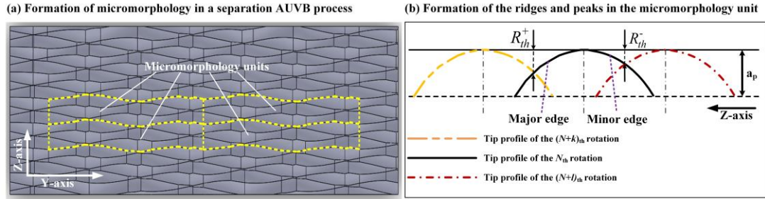
Fig.6 Schematics of the formation of ridges and peaks formed in a separation AUVB process
