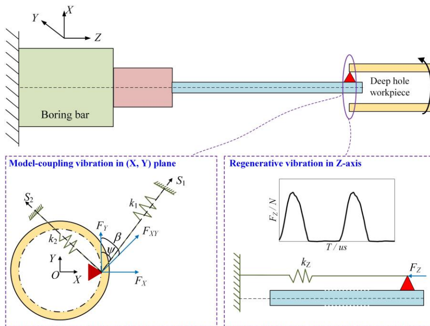
Fig. 5 Vibration model in deep-hole boring
