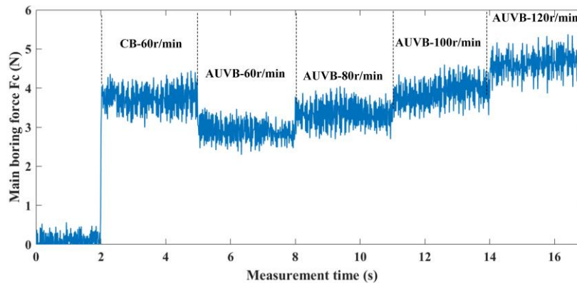
Fig. 12 Boring force signals at different rotational speeds ( D_1=7473 )
