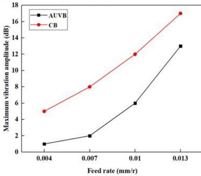
(c) Vibration amplitude (dB) versus feed rate
