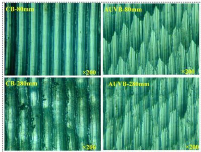
(b) Micrographs of the machined surface
