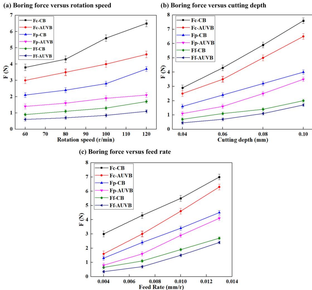
Fig. 10 Influence of machining parameters on boring force ( D_t=7473 )
