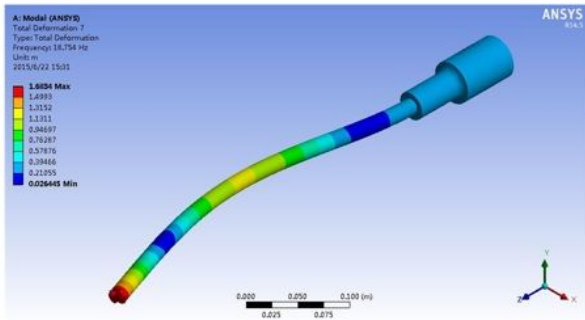
(a) Vibration mode at the frequency of 18.754Hz
