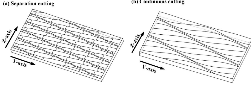
Fig. 5 Simulation results of surface micromorphology in AUVB
