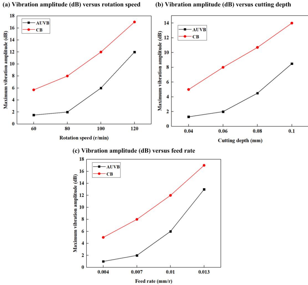
Fig. 19 Influence of machining parameters on vibration amplitude (dB) ( D_l = 7473 )
