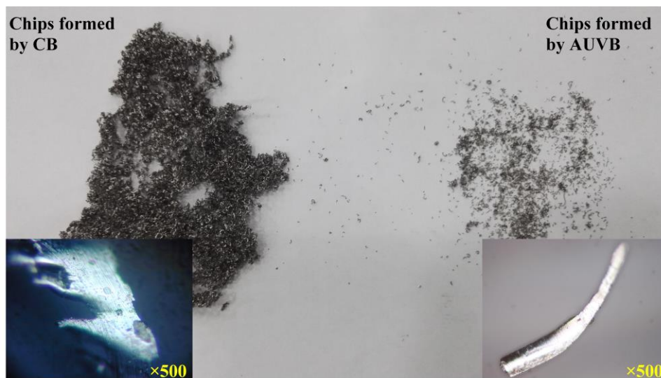
Fig.22 Chip morphologies generated by the CB and the AUVB processes
