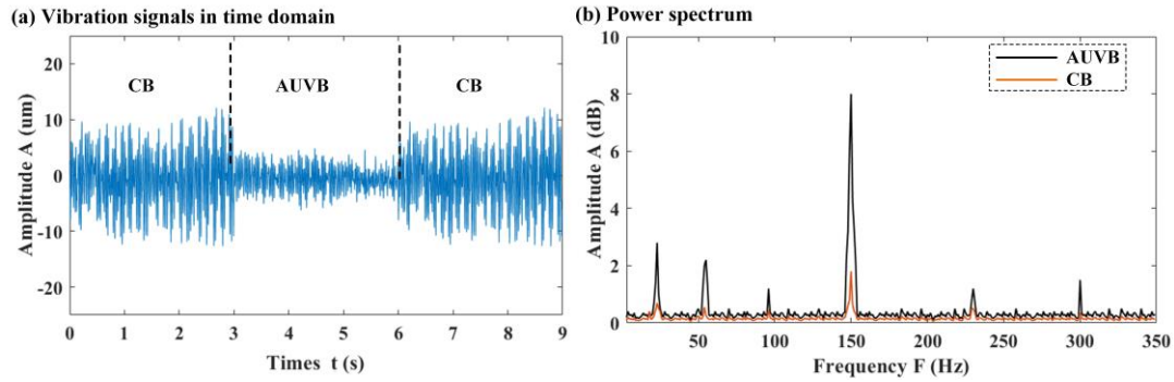
Fig. 17 Vibration signals and power spectrum analysis
