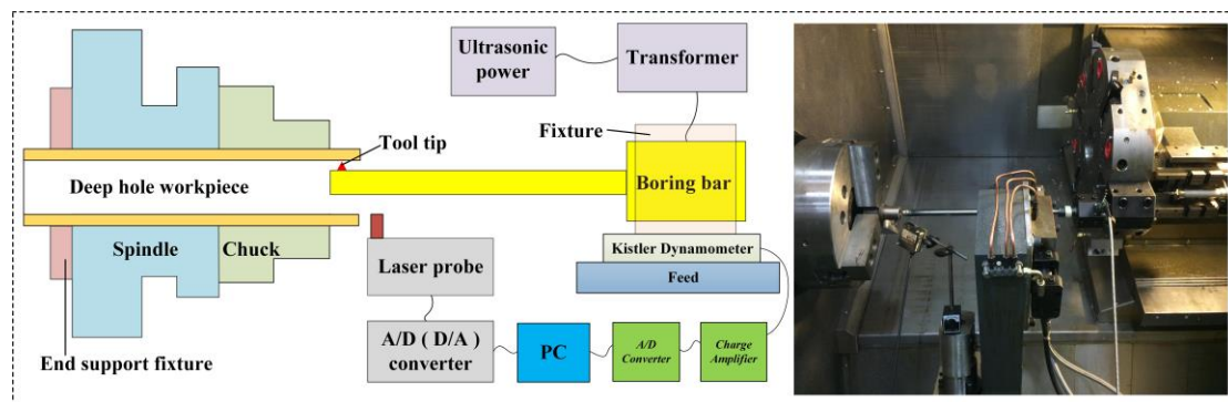
Fig. 9 Schematics of the experiment setup
