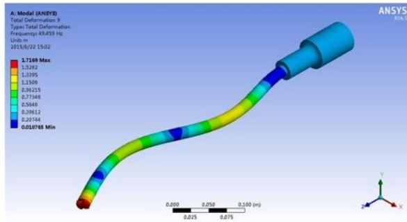
(b) Vibration mode at the frequency of 49.459Hz
