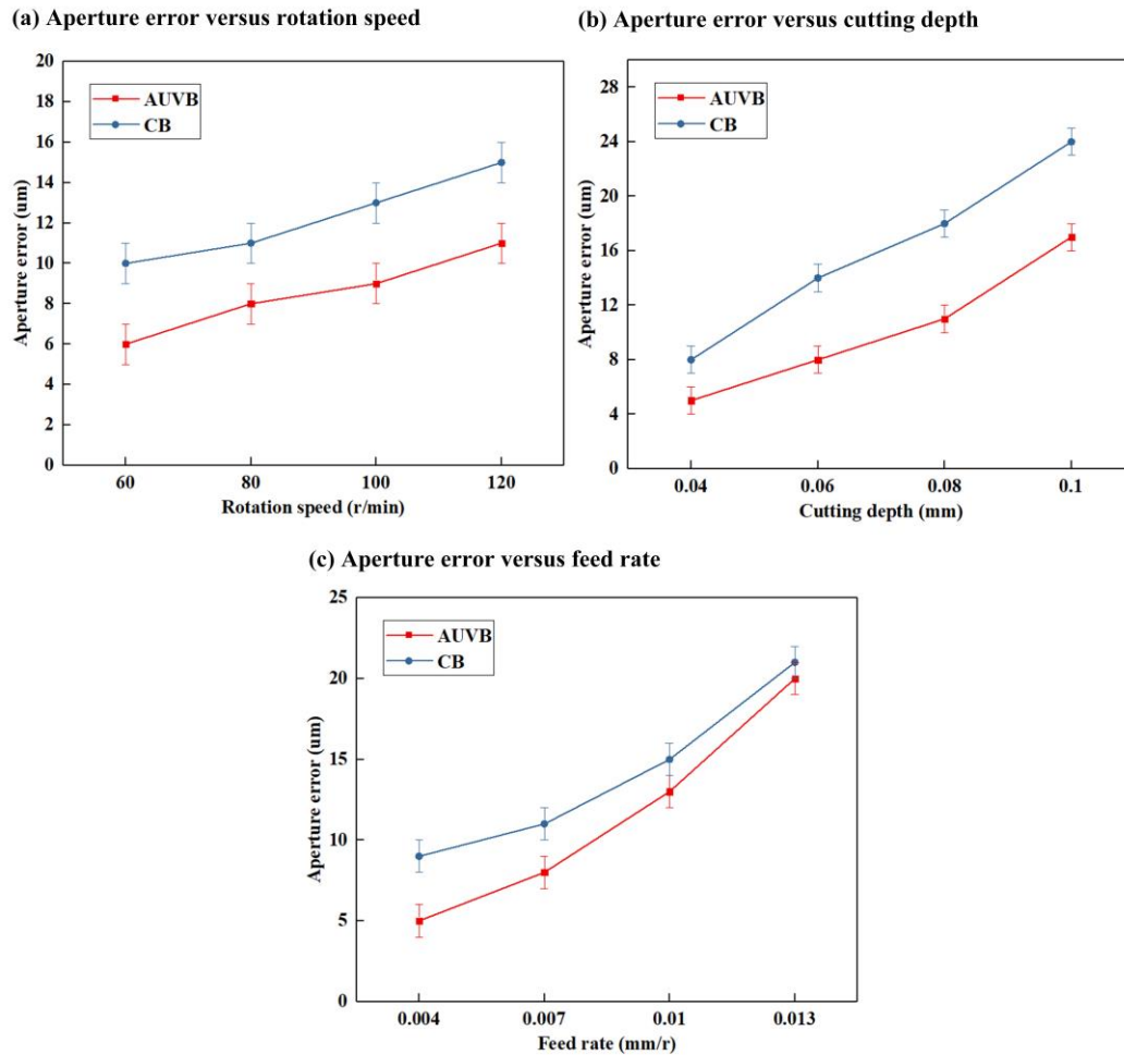
Fig. 15 Influence of machining parameters on boring accuracy ( D_l = 7473 )
