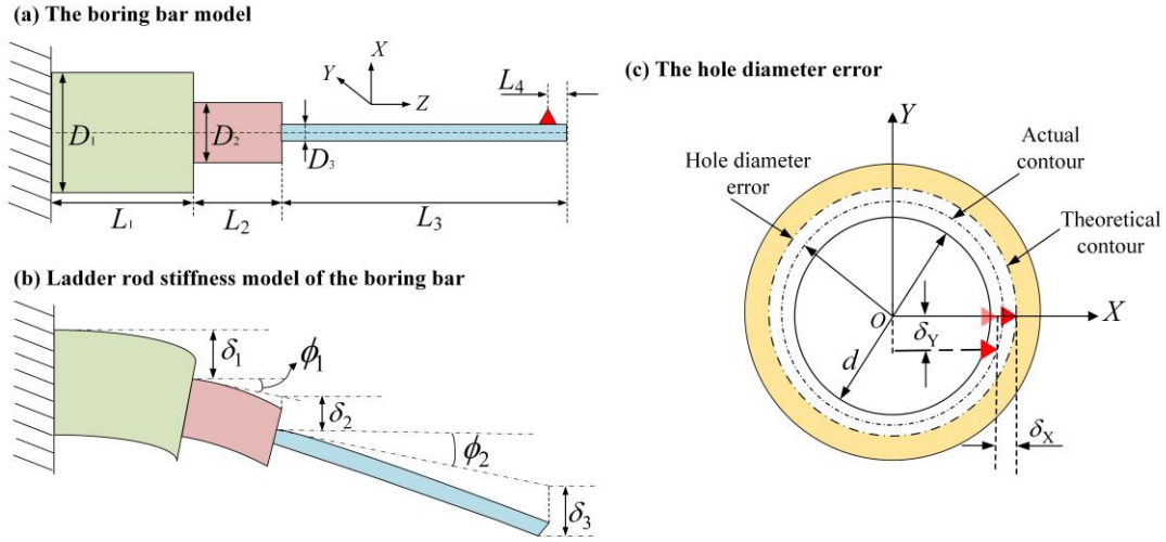
Fig. 3 Static rigidity model and aperture error of ultrasonic vibration-assisted boring bar
