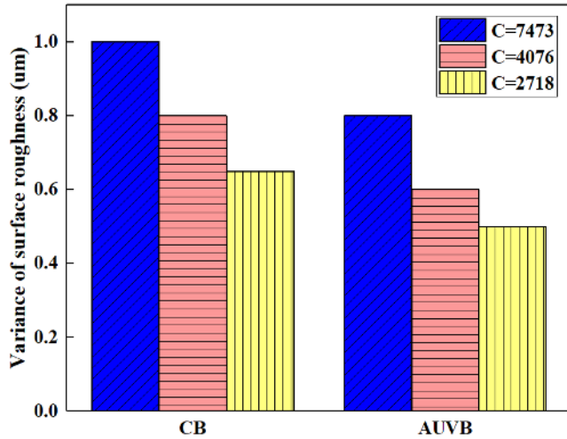
Fig. 24 Impact of size coefficient on surface roughness
