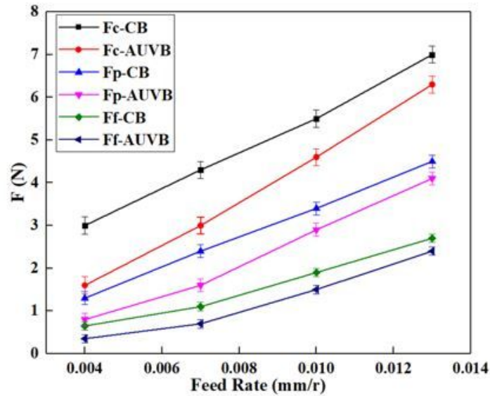
(c) Boring force versus feed rate
