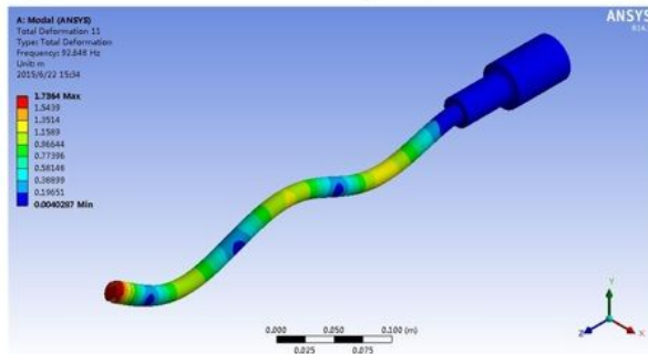
(c) Vibration mode at the frequency of 92.648Hz
