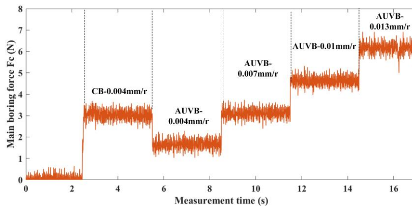
Fig. 13 Boring force signals at different feed rates ( D_1=7473 )
