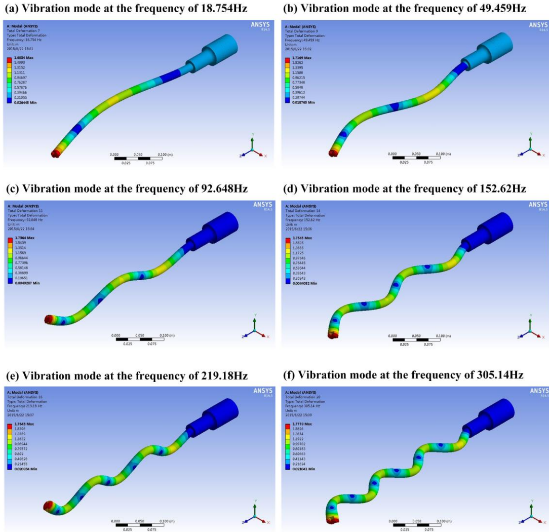
Fig. 18 Vibration modal analysis results for boring bar
