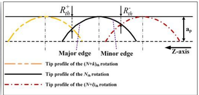
(b) Formation of the ridges and peaks in the micromorphology unit
