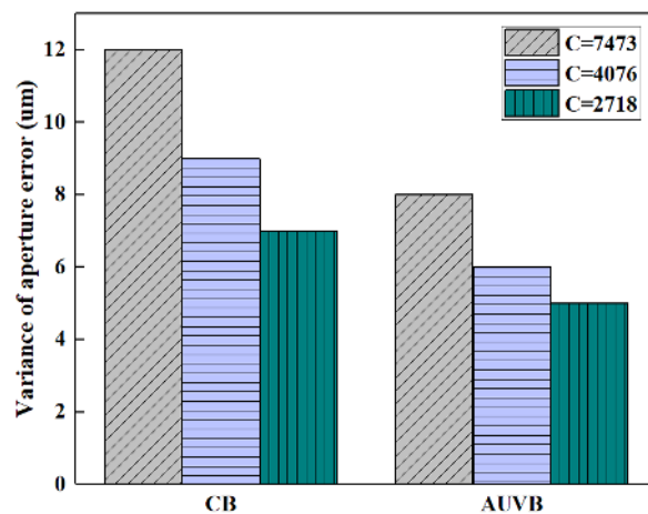
Fig. 16 Influence of size coefficient on boring accuracy
