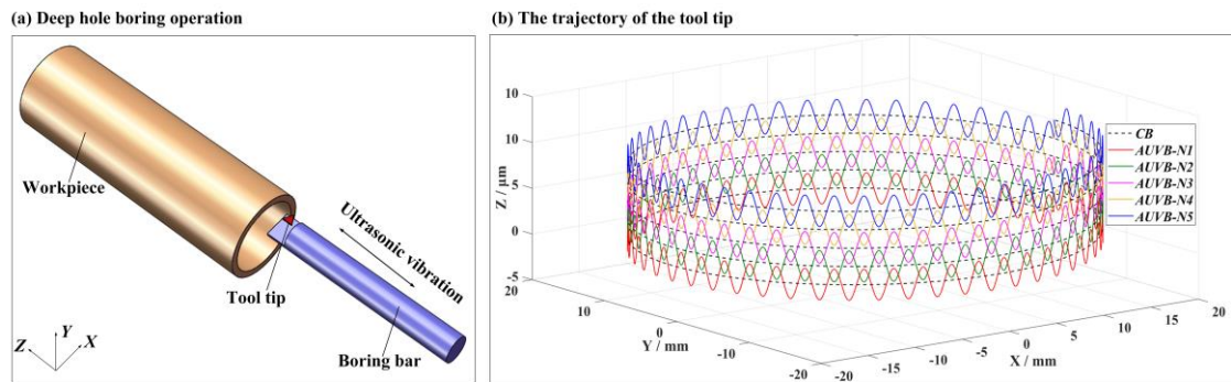
Fig. 1 Schematic of axial ultrasonic vibration-assisted boring
