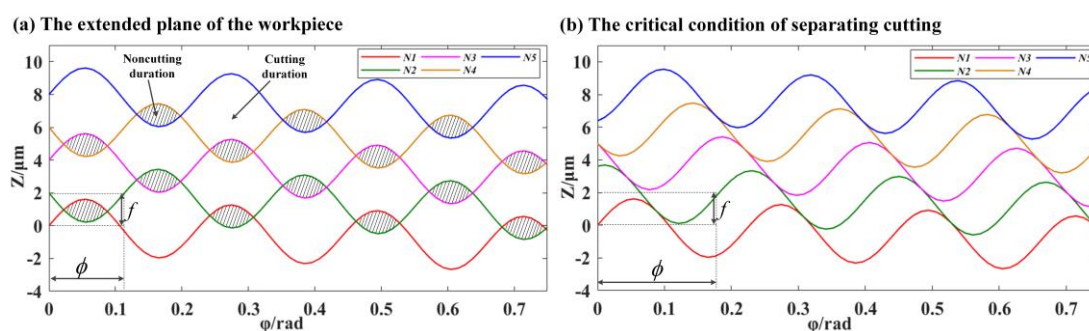
Fig. 2 Separation cutting feature of axial ultrasonic vibration-assisted boring
