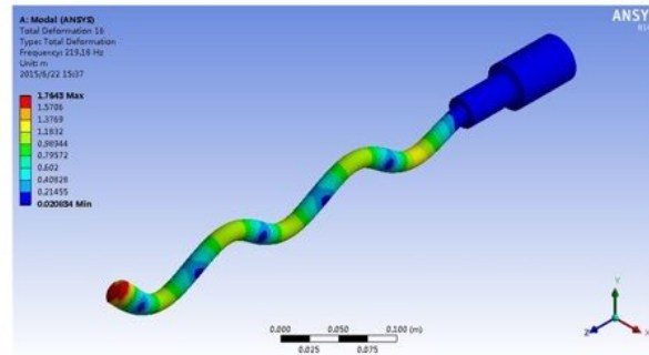
(e) Vibration mode at the frequency of 219.18Hz
