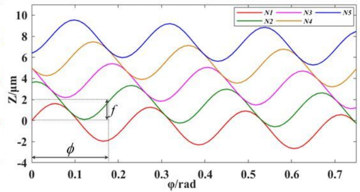
(b) The critical condition of separating cutting
