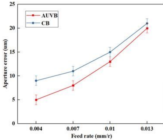
(c) Aperture error versus feed rate
