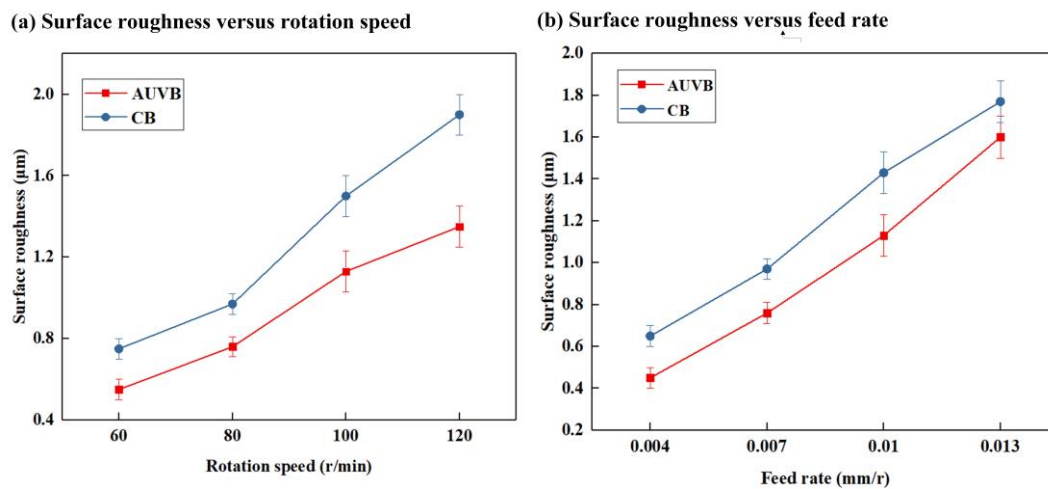
Fig. 23 Influence of rotational speed and feed rate on surface roughness for AUVB ( D_T=4076 )
