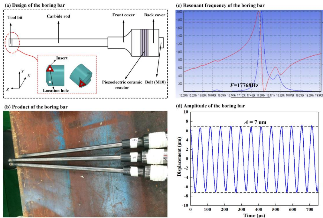
Fig. 8 Design and implementation of the boring bar
