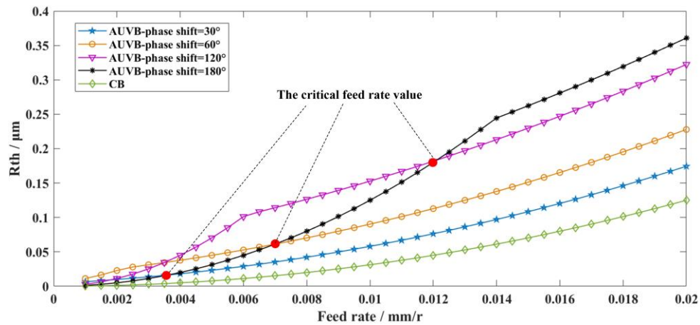
Fig. 7 The height of peaks as formed in the AUVB and the CB process
