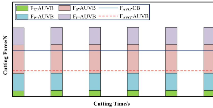
Fig. 11 Schematic of cutting force reduction principle for AUVB
