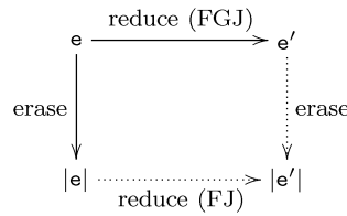
Fig. 9. Commuting diagram.
