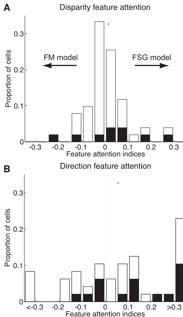
Fig. 4. Population attention indices testing the feature-similarity gain (FSG) model for feature-based attention for binocular disparity and direction of motion. Attention indices for each feature: binocular disparity (A) and direction of motion (B) calculated with the null value of each feature in the receptive field. Arrow on each plot signifies the population mean; black portions signify significant cells as determined by Wilcoxon test. A shift to the left would provide support for the feature matching (FM) model; a shift to the right would provide support for the FSG model. n = 44 .
