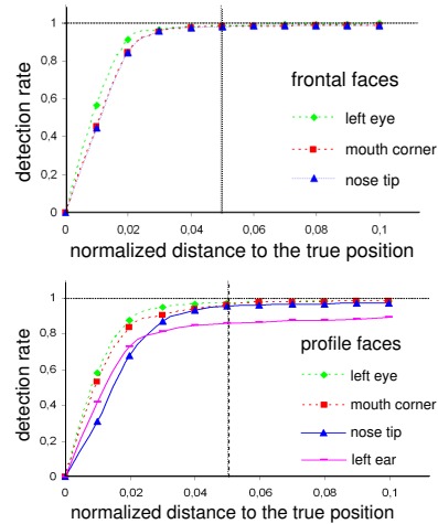
Fig. 6. Detection performance of the facial feature classifiers. With a threshold of 0.05 for the distance between the estimated feature position and the true position in a normalized face bounding box, we achieve a detection rate of 98%.
