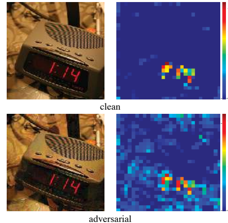
Figure 1. Feature map in the res_3 block of an ImageNet-trained ResNet-50 [9] applied on a clean image (top) and on its adversarially perturbed counterpart (bottom). The adversarial perturbation was produced using PGD [16] with maximum perturbation \epsilon = 16 (out of 256). In this example, the adversarial image is incorrectly recognized as “space heater”; the true label is “digital clock”.
