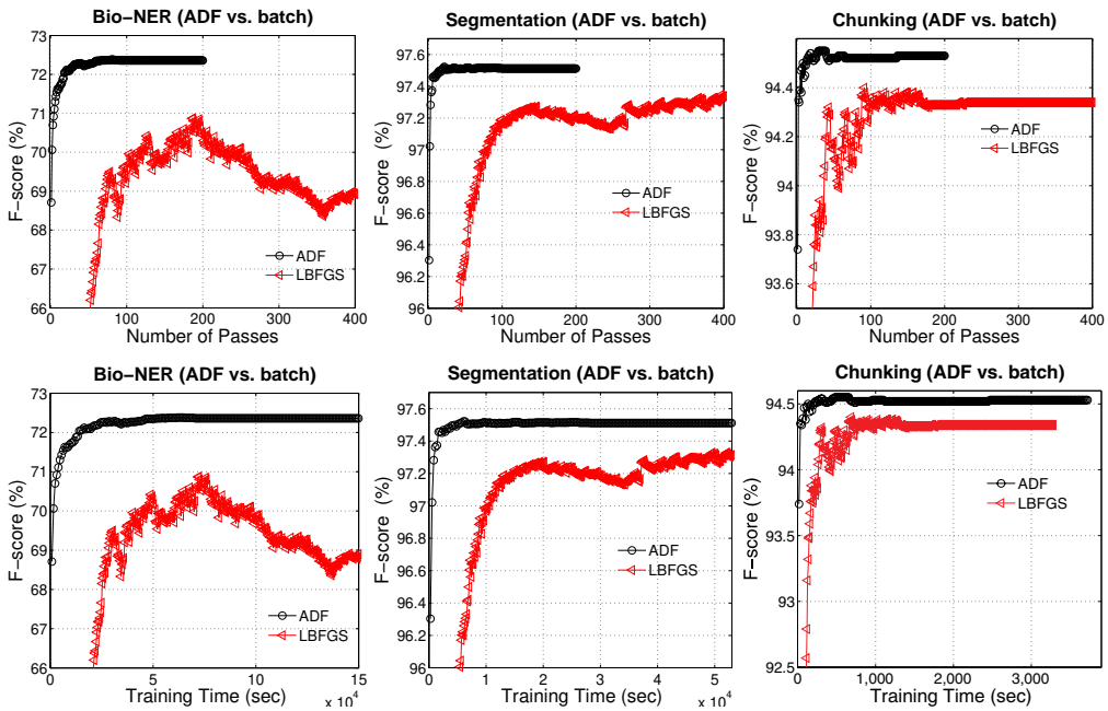
Figure 4 Comparisons between the ADF method and the batch training method LFBGS. (Top Row) Comparisons based on training passes. As we can see, the ADF method converges much faster than the LFBGS method, and with better accuracy on the convergence state. (Bottom Row) Comparisons based on wall-clock time.
