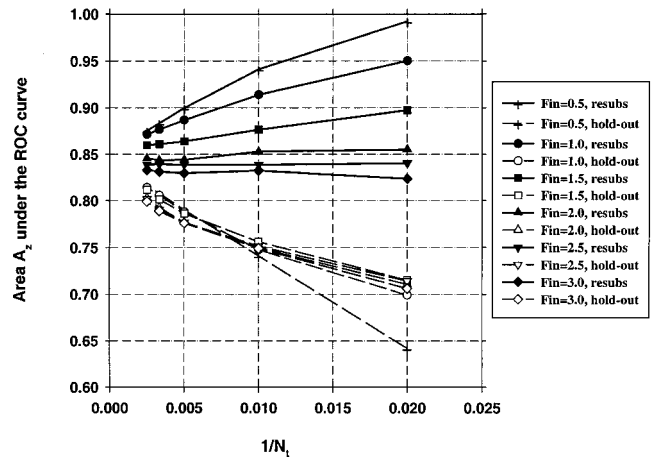
FIG. 18. Case 3(a) (an example from CAD, no diagonalization), A_2(\infty) = 0.86 . Feature selection from the design samples. Total sample size N_s = 500 samples per class. The area A_2 under the ROC curve versus the inverse of the number of design samples N_t per class. Feature selection was performed using an input feature space of M = 100 available features.
