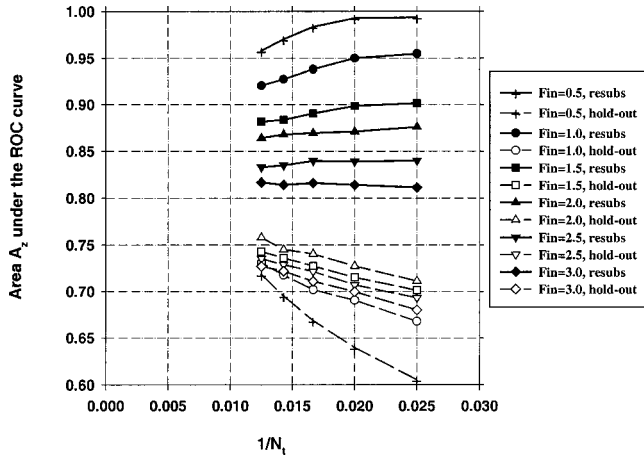
FIG. 17. Case 3(a) (an example from CAD, no diagonalization), A_2(\infty) = 0.86 . Feature selection from the design samples. Total sample size N_s = 100 samples per class. The area A_2 under the ROC curve versus the inverse of the number of design samples N_t per class. Feature selection was performed using an input feature space of M = 100 available features.
