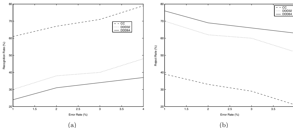
Fig. 6 Performance of the classifiers on the test set for error rates varying from 1 to 4%. a Trade-off between recognition rate and error rate. b Trade-off between reject rate and error rate
