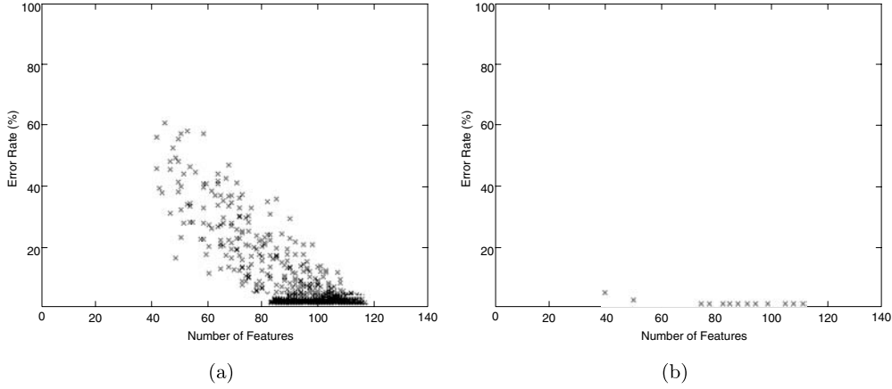
Fig. 8 Feature selection using the weighted-sum approach. a Evolution of the population in the objectives plane (one trial) and b Pareto-optimal solutions found by the classical approach after several trials
