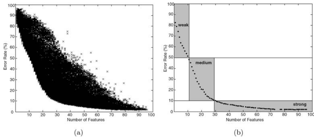
Fig. 7 Supervised feature selection using a Pareto-based approach. a Evolution of the population in the objective plane, b Pareto-optimal front and its different classes of classifiers
