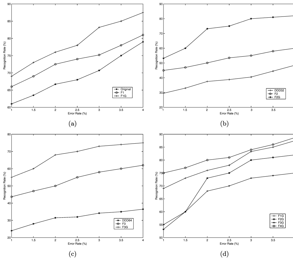
Fig. 14 Improvements yielded by the ensembles: F_1 a, F_2 b, F_3 c, and comparison among all ensembles d
