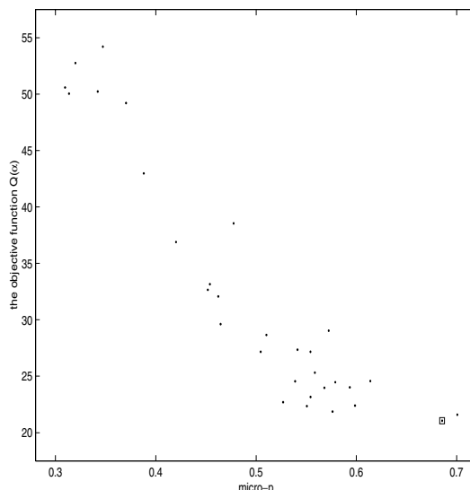
Figure 5. For the Newsgroups data set and for k = 10 , we plot the objective function Q(\alpha) versus micro- p values for all the feature weightings in figure 4. The micro- p value corresponding to optimal feature weighting is distinguished by putting the symbol \square around it. The “negative correlation” between the objective function and micro- p values is clearly evident from the plot.
