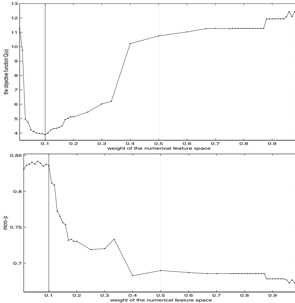
Figure 3. For the AUSTRALIAN data and for k = 8 , the top panel (resp. bottom panel) shows a plot of the objective function (resp. micro- p values) versus the weight of the numerical feature space. The solid (resp. dotted) vertical line indicate the position of the optimal feature weighting (resp. the uniform feature weighting). The “negative correlation” between the objective function and micro- p values is clearly evident from the plots. Finally, superiority of the optimal feature weighting over the uniform feature weighting is also evident.
