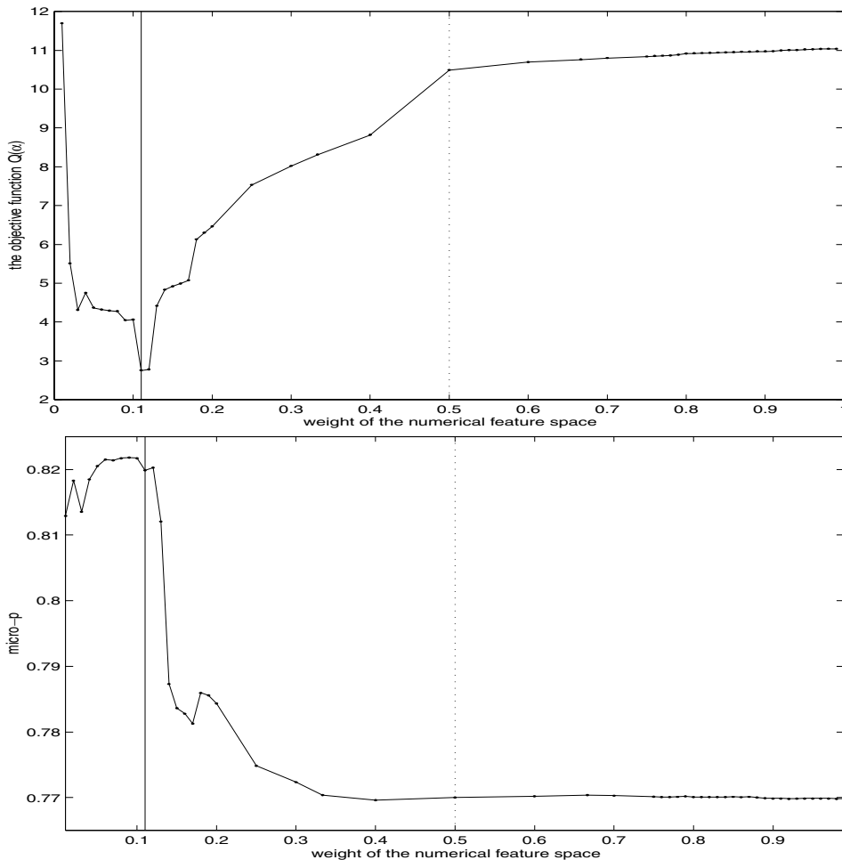
Figure 2. For the ADULT data and for k = 8 , the top panel (resp. bottom panel) shows a plot of the objective function (resp. micro- p values) versus the weight of the numerical feature space. The solid (resp. dotted) vertical line indicate the position of the optimal feature weighting (resp. the uniform feature weighting). The “negative correlation” between the objective function and micro- p values is clearly evident from the plots. Finally, superiority of the optimal feature weighting over the uniform feature weighting is also evident.
