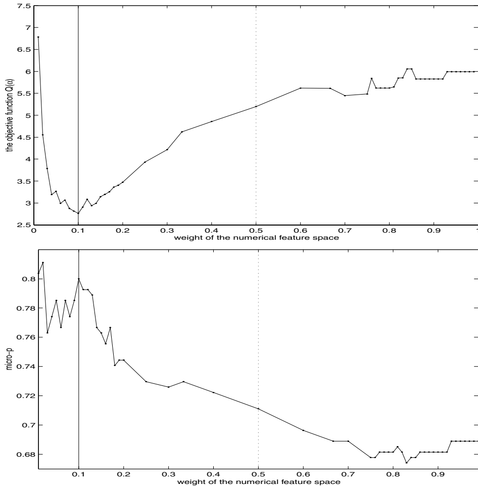
Figure 1. For the HEART data and for k = 8 , the top panel (resp. bottom panel) shows a plot of the objective function (resp. micro- p values) versus the weight of the numerical feature space. The solid (resp. dotted) vertical line indicate the position of the optimal feature weighting (resp. the uniform feature weighting). The “negative correlation” between the objective function and micro- p values is clearly evident from the plots. Finally, superiority of the optimal feature weighting over the uniform feature weighting is also evident.
