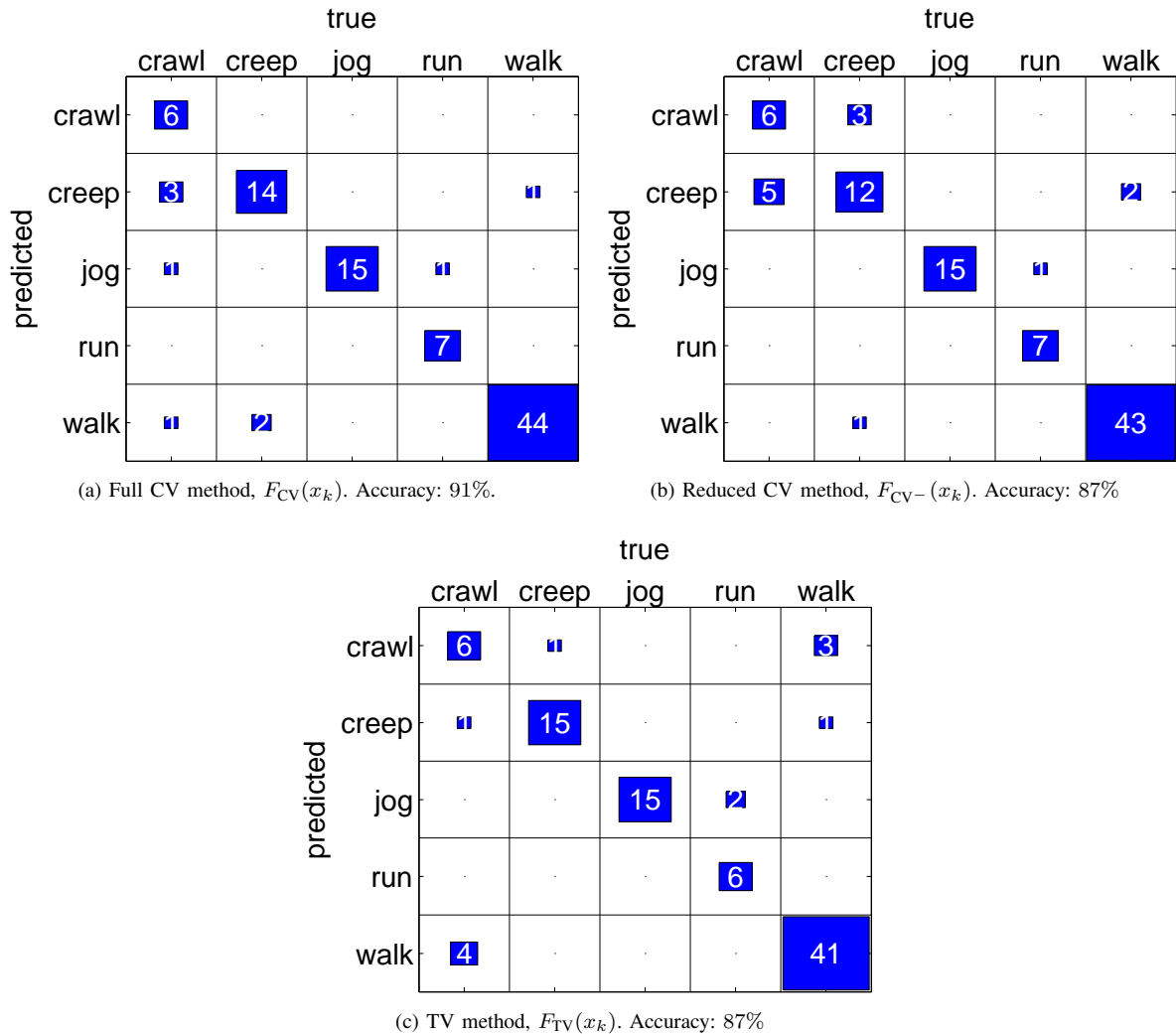
Fig. 5: Classification results derived using ‘leave-one-sequence-out’ validation with 95 instances of data. The numbers in the boxes are the samples classified that way.
