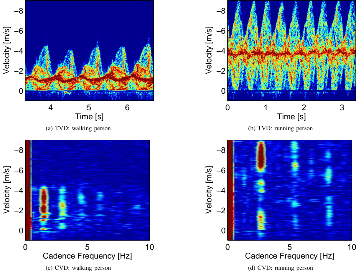
Fig. 1: Time-velocity diagrams (TVD) and corresponding cadence-velocity diagrams (CVD) for persons walking and running.
