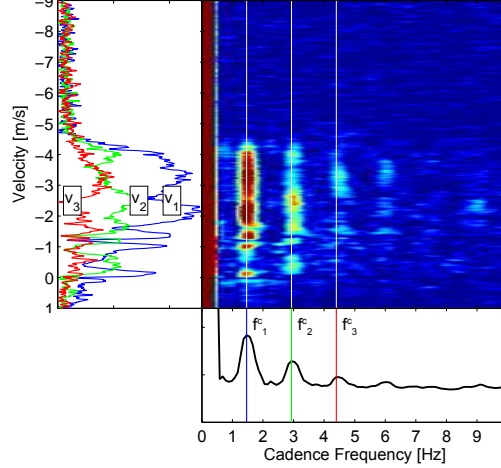
Fig. 4: CV based feature extraction. A CVD with some of the features in the CV method illustrated (cadence frequencies and velocity profiles).
