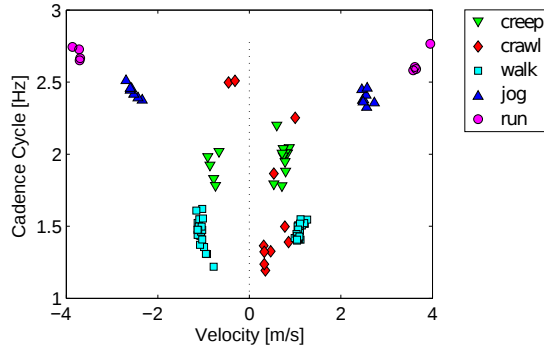
Fig. 2: The distribution of base velocity and limb cadence frequency for all targets within the dataset.
