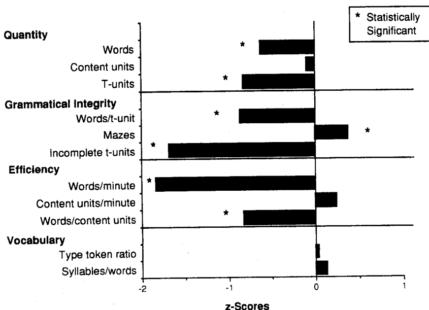
FIGURE 1. Mean z -scores of subjects with ALS and dysarthria as compared to controls for selected measures of spontaneous language production. Asterisks indicate measures for which the groups are significantly different.
