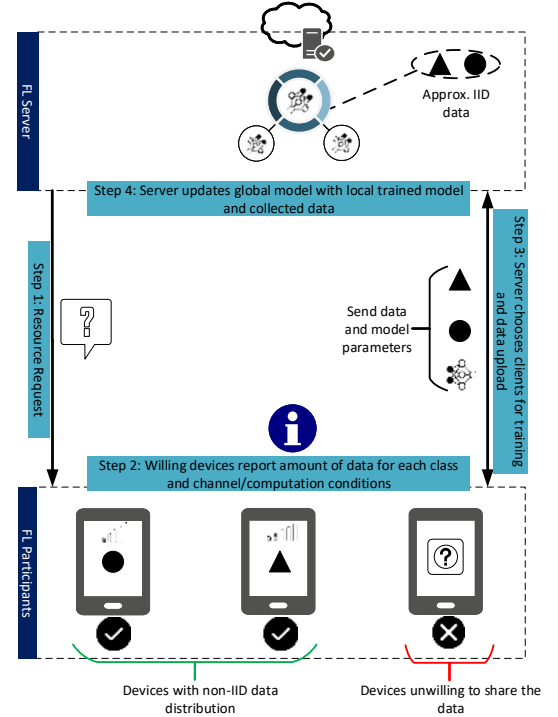
Fig. 7: Participant selection under FedCS and Hybrid-FL protocols.
