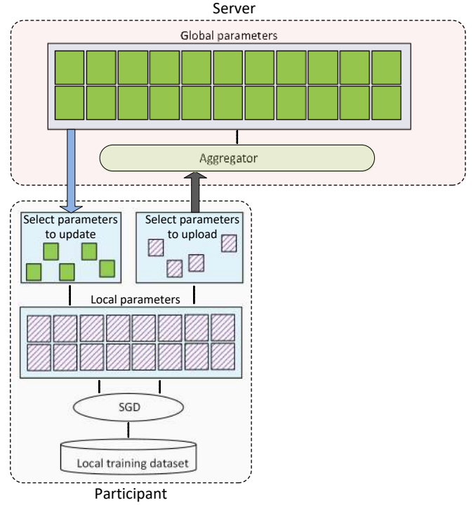
Fig. 11: Selective parameters sharing model.
