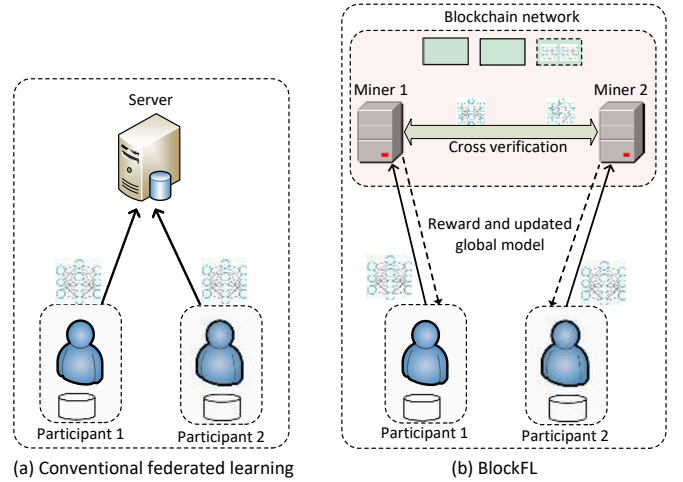
Fig. 13: An illustration of (a) conventional FL and (b) the proposed BlockFL architectures.
