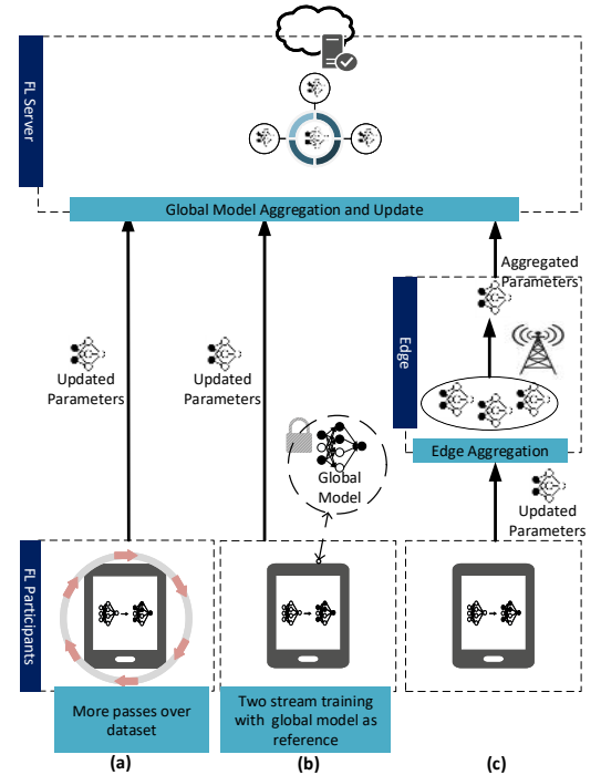
Fig. 5: Approaches to increase computation at edge and end devices include (a) Increased computation at end devices, e.g., more passes over dataset before communication [23], [98] (b) Two-stream training with global model as a reference [99] and (c) Intermediate edge server aggregation [100].
