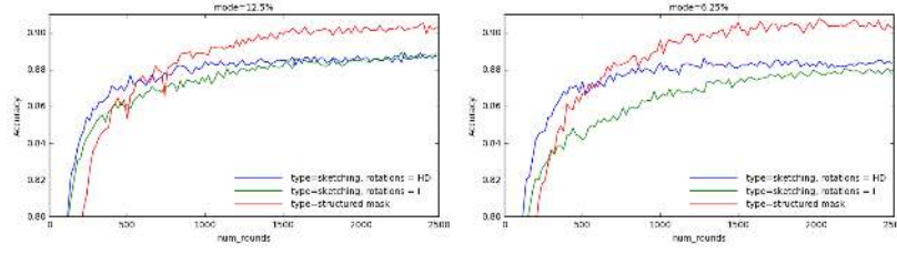
Figure 2: Comparison of structured random mask updates and sketched updates without quantization on the CIFAR data.
