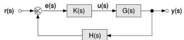
FIG. 14. Block diagram of feedback system with nontrivial sensor dynamics, given by H(s) .
