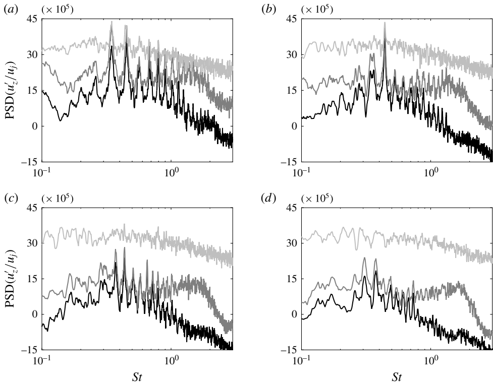
FIGURE 8. Power spectral densities (PSD) of axial velocity fluctuations u'_z obtained at r = r_0 , at \text{---} z = 0.25r_0 , \text{---} z = r_0 and \text{---} z = 4r_0 , as a function of St , in dB/ St : (a) JetL6, (b) JetL8, (c) JetL10 and (d) JetL12.
