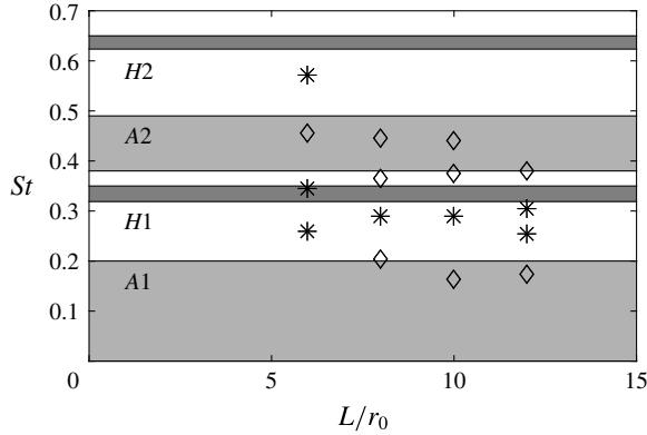
FIGURE 17. Representation of the tone Strouhal numbers as a function of the nozzle-to-plate distance: LES tone frequencies associated with \diamond axisymmetric and * helical modes and allowable frequency ranges of the upstream-propagating neutral acoustic wave modes in an ideally expanded round jet at \mathcal{M}_j = 1.5 .
