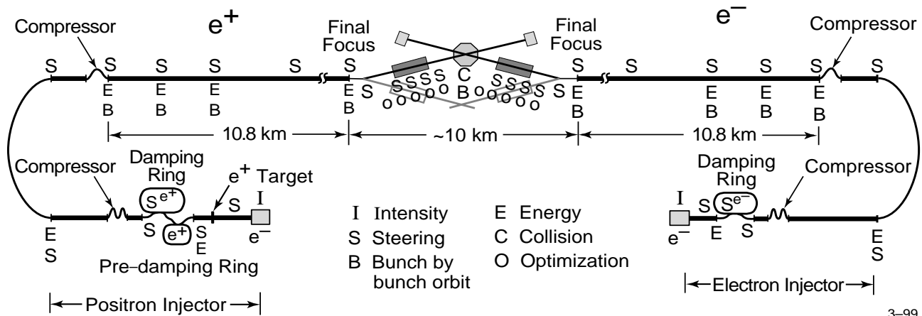
Fig 2: NLC Schematic with Feedback Loops Shown
