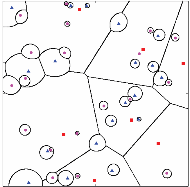
Fig. 4. Unbiased Cell Association in a 3-tier Heterogeneous Network
