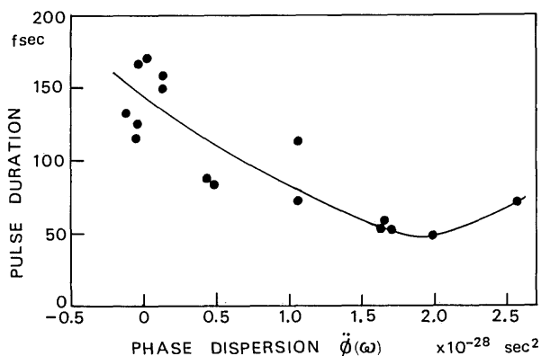
Fig. 2. Generated pulse duration as a function of cavity-mirror dispersion \ddot{\phi}(\omega) .
