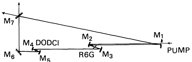
Fig. 1. Cavity configuration of the CPM laser used in the experiment. The focusing mirrors around the amplifying and absorbing jets are, respectively, M_2 and M_3 ( R_c = 10 cm) and M_4 and M_5 ( R_c = 2.5 cm). The perimeter of the cavity is 325 cm.
