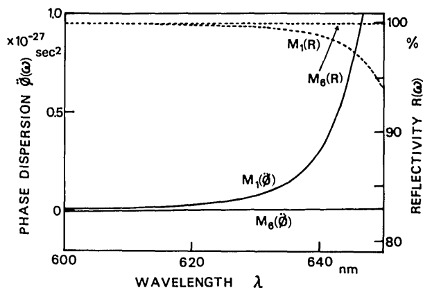
Fig. 4. The second derivative \ddot{\phi}(\omega) of the phase shift and the reflectivity R(\omega) plotted against the wavelength for mirrors M_1 and M_6 for the configuration used in the generation of the shortest pulse.
