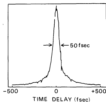
Fig. 3. Autocorrelation function of pulses from the CPM laser with chirp compensation by a cavity mirror. The full width at half-maximum corresponds to a sech 2 pulse duration of 50 fsec.
