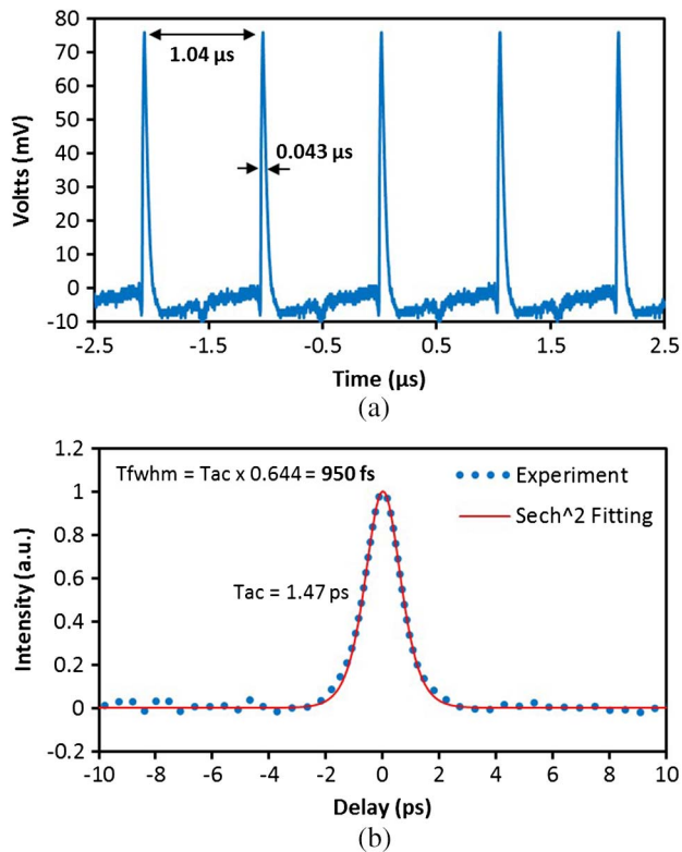
Fig. 6. (a) Oscilloscope train at a pump power of 165 mW. (b) The autocorrelation trace.
