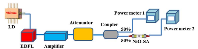
Fig. 2. Modulation depth measurement setup.
