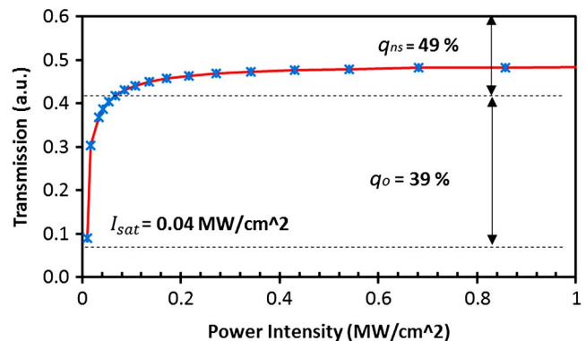
Fig. 3. Nonlinear optical absorption characteristics of the NiO-SA.
