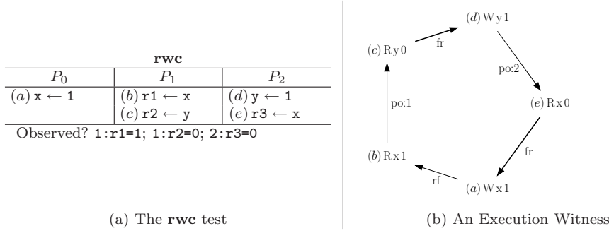
Fig. 13 The wrc Test and a Candidate Execution
