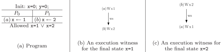
Fig. 4 A program and its two different write serialisations
