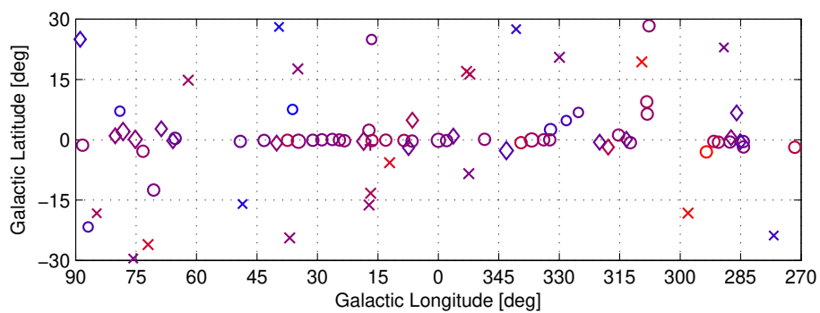
Fig. 11.— The LAT Bright Source List, showing the locations of sources in the inner Galaxy. The legend is the same as in Figure 10.
