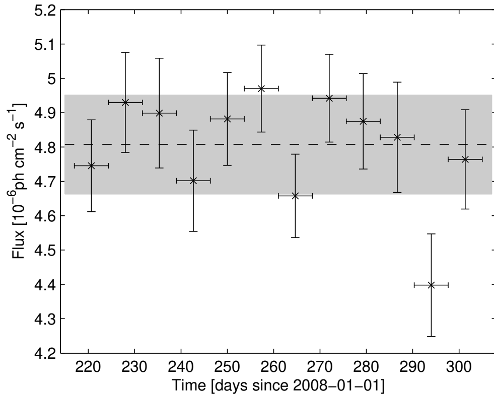
Fig. 6.— Same as Figure 5 for Geminga (0FGL J0634.0+1745).
