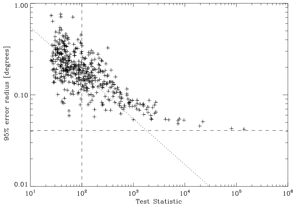
Fig. 3.— Source location error radii ( r_{95} from Eq. 1) as a function of their Test Statistic (Sect. 3.3), down to a limit of TS = 25 . The dotted line is a 1/\sqrt{TS} trend for reference. The vertical dashed line is our TS = 100 threshold. The horizontal dashed line is the systematic error that we adopted.
