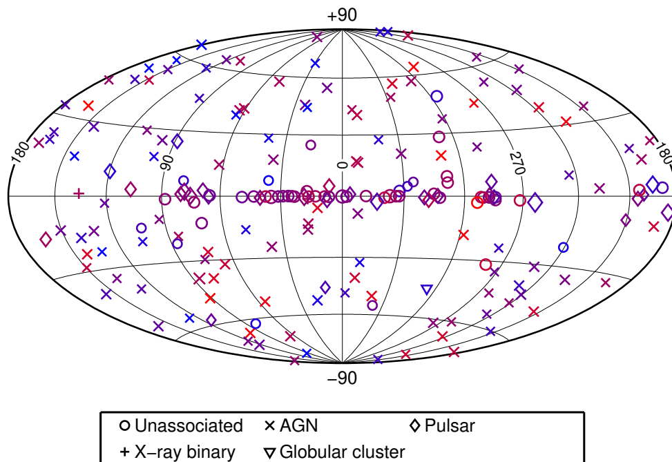
Fig. 10.— The LAT Bright Source List, showing the locations on the sky (Galactic coordinates in Aitoff projection) coded according to the legend. Symbols in blue indicate sources with harder spectra than those in red.
