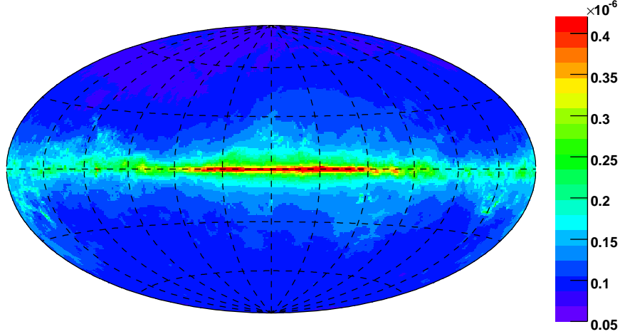
Fig. 4.— Flux ( E > 100 MeV) needed for a 10\text{-}\sigma detection for the LAT data for the 3-month time range considered in this paper. The assumed photon spectral index is 2.2. Galactic coordinates.
