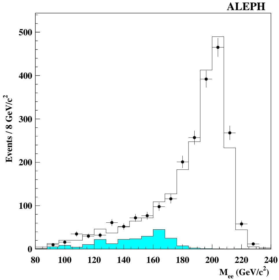
Figure 13: The M_{e+e-} distribution for electron-pair events collected at \sqrt{s} = 207 \text{ GeV} in the angular range -0.9 < \cos \theta < 0.7 . The data (dots) are compared to the Monte Carlo expectation (histogram). The filled area shows the background contribution.
