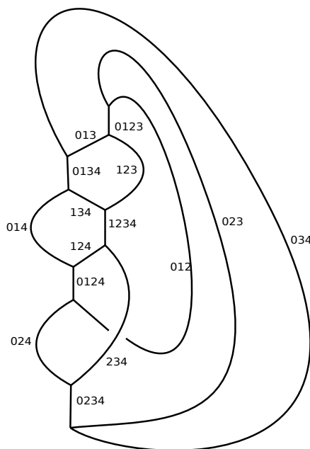
Figure 2. This image, essentially a reproduction of figure 16 from [35], represents the boundary of the 4-simplex, considered as a triangulation of the 3-sphere. We have flattened the image onto the page using a framing induced from the branching structure, which gives us a labeling of vertices 0 through 4. This picture is actually Poincaré dual in the 3-sphere to that 4-simplex, with (most) edges here representing triangles of the vertex-ordered 4-simplex. This is so the graph depicts the labeling of triangles in X by line objects. Representing triangles, these edges are labeled by triples of vertices, and there are 5 choose 3 of those. There are some extra edges where we have resolved 4-way intersections to make the graph trivalent. These are labeled by tetrads of vertices and coincide with the 5 choose 4 tetrahedra of the dual 4-simplex. The state sum gives us a labeling of these edges by 1 , \psi , and \sigma , and the rules of the Ising braided fusion category of [6] gives us a way to evaluate this picture to a number. This defines the 15j symbol.
