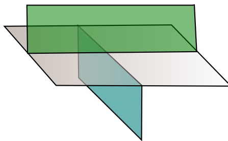
Figure 1. A picture of the F-junction or A_3 singularity, where four zippers meet. With the x axis along the blue-grey junction and the y axis along the green-grey junction, the planes x + y = c cut through this picture to give a movie of the F move as we vary c through zero.
