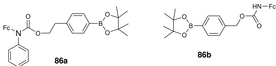
Figure 33. Chemical structure of aminoferrocene-based derivatives ( 86a–b ).
