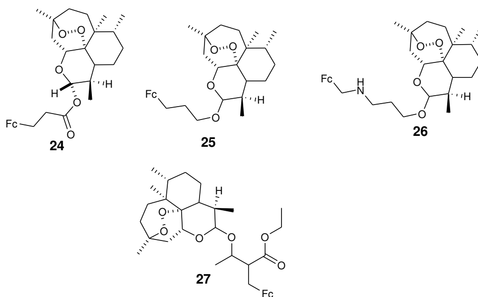
Figure 10. Chemical structures of dihydroartemisinin ferrocene derivatives (24–27).
