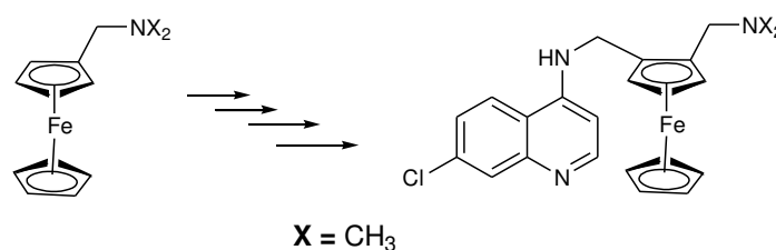
Figure 1. Synthesis of ferroquine by Biot and co-partners.
