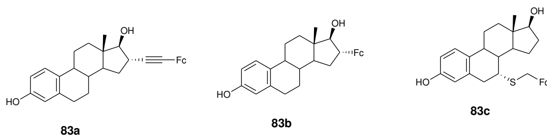
Figure 30. Hybrid compounds 83a–c.
