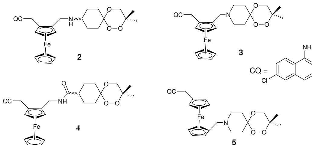
Figure 3. Chemical structures of trioxaferroquine derivatives ( 2-5 ).
