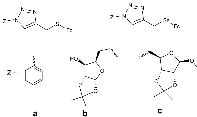
Figure 24. Chemical structures of ferrocenyl-chalcogeno-triazole conjugates (70–71).
