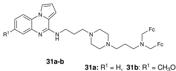
Figure 12. Structure of synthesized ferrocenyl pyrrolo[1,2-a]quinoxaline derivatives ( 30a–b and 31a–b ).
