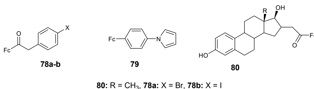
Figure 27. Chemical structures of ferrocene-carboxylate derivatives (76–80).
