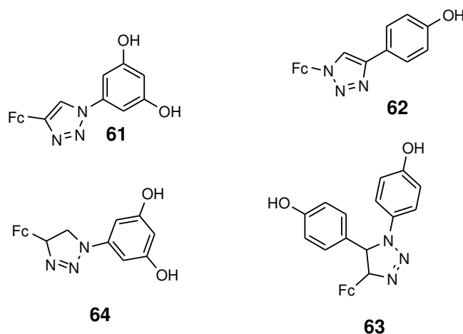
Figure 21. Chemical structures of hydroxyphenyl-ferrocephenol derivatives ( 61–64 ).
