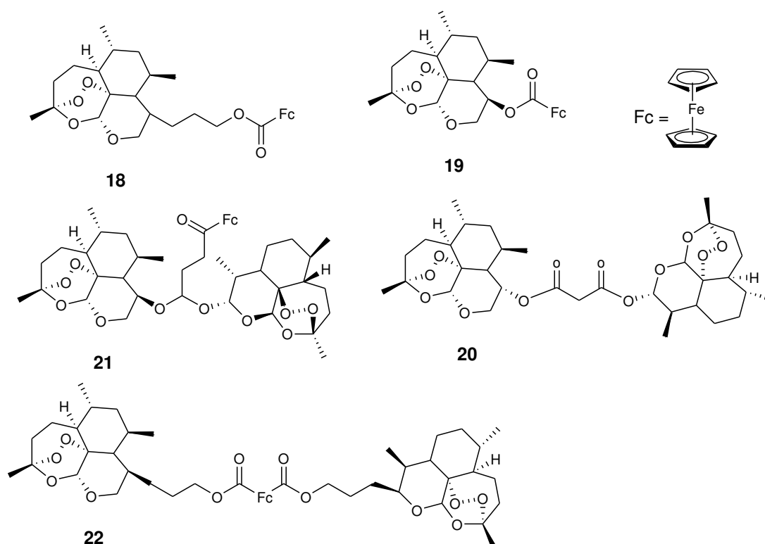
Figure 8. Chemical structures of second generation dihydroartemisinin ferrocene derivatives (18–22).
