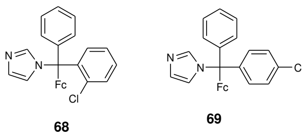
Figure 23. Chemical structures of ferrocenyl-clotrimazole derivatives (68–69).
