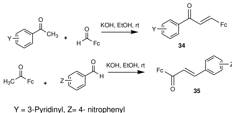
Figure 15. Ferrocenyl chalcones derivatives (34–35).
