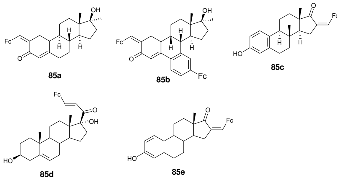
Figure 32. Chemical structures of ferrocene-steroids derivatives ( 85a–e ).
