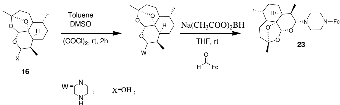
Figure 9. Synthesis of amino-artemisinin-ferrocene compound (23).
