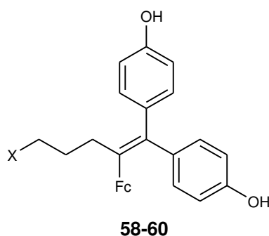
58: X = OH 59: X = O-C(=O)- 60: X = O-C(=O)Ph
