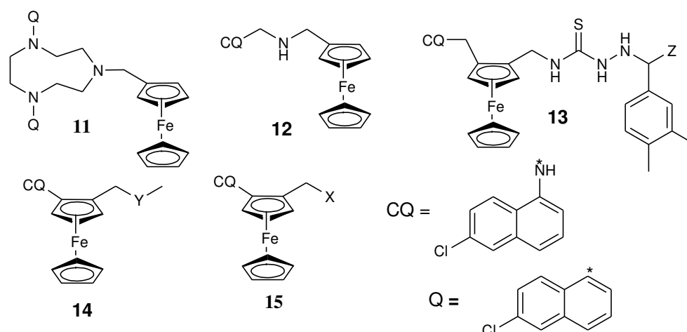
Figure 5. Chemical structures of quinolone-ferrocene hybrids ( 11–15 ). 13-Z = CH 3 , 14-Y = 1,2,3,5-diisopropylidene glucofuranose moiety, 15a-X = diisopropylidene-protected 6-amino-deoxyglucofuranose, 15b-X = 6-amino-6-deoxygalactopyranose.
