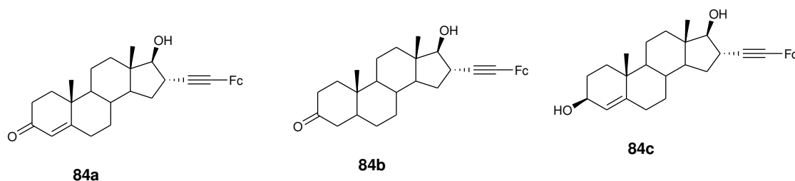
Figure 31. Hybrid compounds 84a–c.
