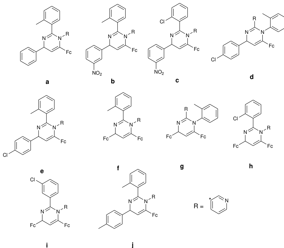
Figure 26. Chemical structures of ferrocene with 1,4-dihydropyrimidine derivatives (75a–j).
