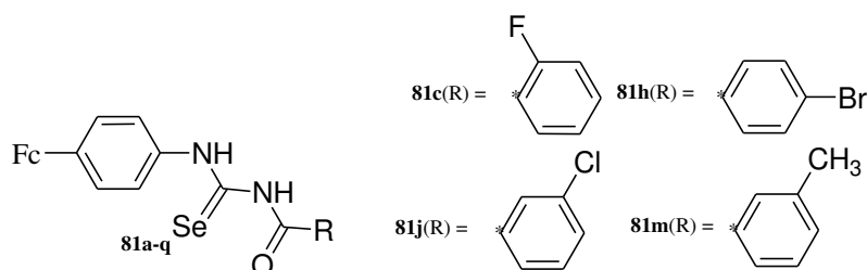
Figure 28. Chemical structures of ferrocene incorporated selenourea derivatives ( 81a–q ).
