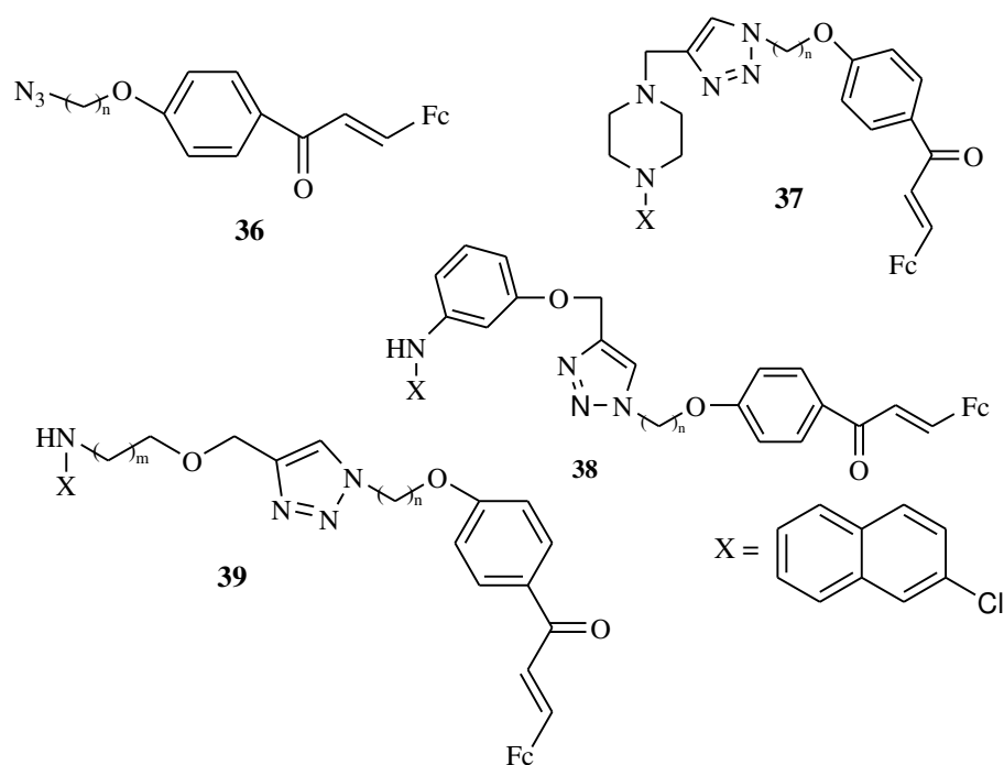
Figure 16. Chemical structures of O -alkyl azide ferrocenylchalcones ( 36 ); piperazine ( 37 ), phenyl ( 38 ), amino alcohol ( 39 )-linked 7-chloroquinoline-ferrocenylchalcone derivatives.
