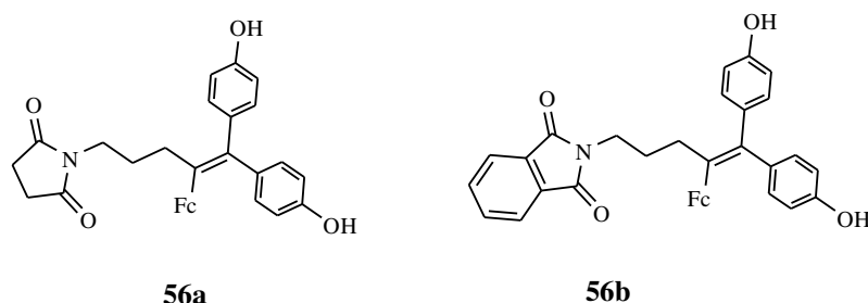
Figure 18. Hybrids 56a and 56b .
