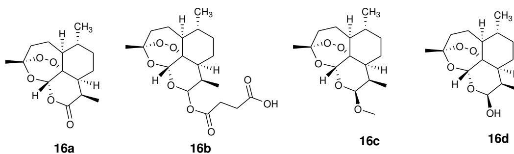
Figure 6. Artemisinin and its derivatives.
