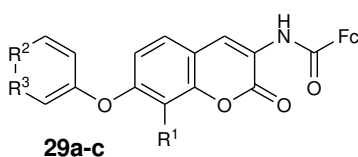
29a: R 1 = H; R 2 = NMe; R 3 = CH 2 29b: R 1 = H; R 2 = CH 2 ; R 3 = NMe 29c: R 1 = Me; R 2 = NMe; R 3 = CH 2
