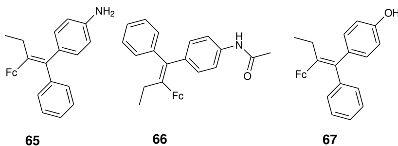
Figure 22. Chemical structures of 2-ferrocenyl-1-1-diphenyl-but-1-ene derivatives ( 65–67 ).
