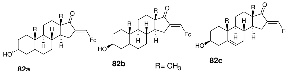
Figure 29. Hybrid compounds 82a–c.
