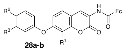
28a: R 1 = H; R 2 = Bu; R 3 = H 28b: R 1 = H; R 2 = OMe; R 3 = H
