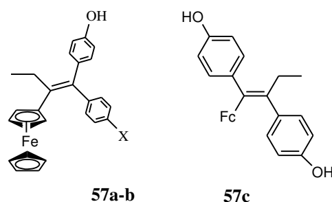
57a: X = OH ; 57b: X = O(CH 2 ) 3 N(CH 3 ) 2
