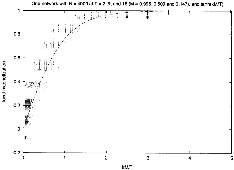
Fig. 2. Correlation between the number of neighbours and the local magnetization \langle S_i \rangle for one network of N = 4000 at T = 2, 9 and 16 . Average over 250 < t \leq 500 iterations. The curve is the mean field prediction \tanh(\beta k M) . N = 2,000,000 gives similar effects.
