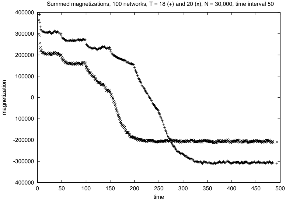
Fig. 3. Total magnetization versus time, summed over 100 networks of N = 30,000 when after every 50 iterations the most-connected free spin is forced down permanently. For lower temperatures, the sign change of the magnetization happens later. N = 2,000,000 gives similar effects.
