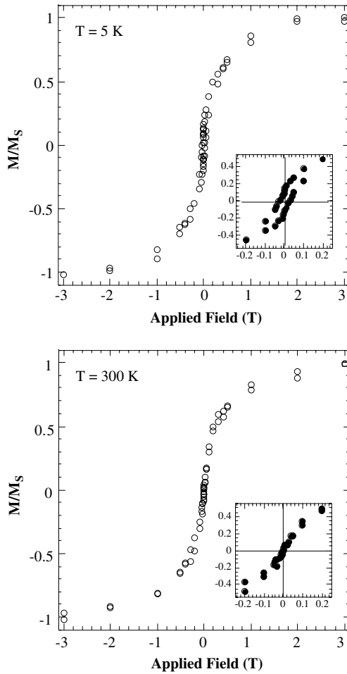
Fig. 1. Normalized magnetization loops at 5 K (top) and 300 K (bottom) for field applied parallel to the plane of a ZnO sample implanted with 3 at.% Co.
