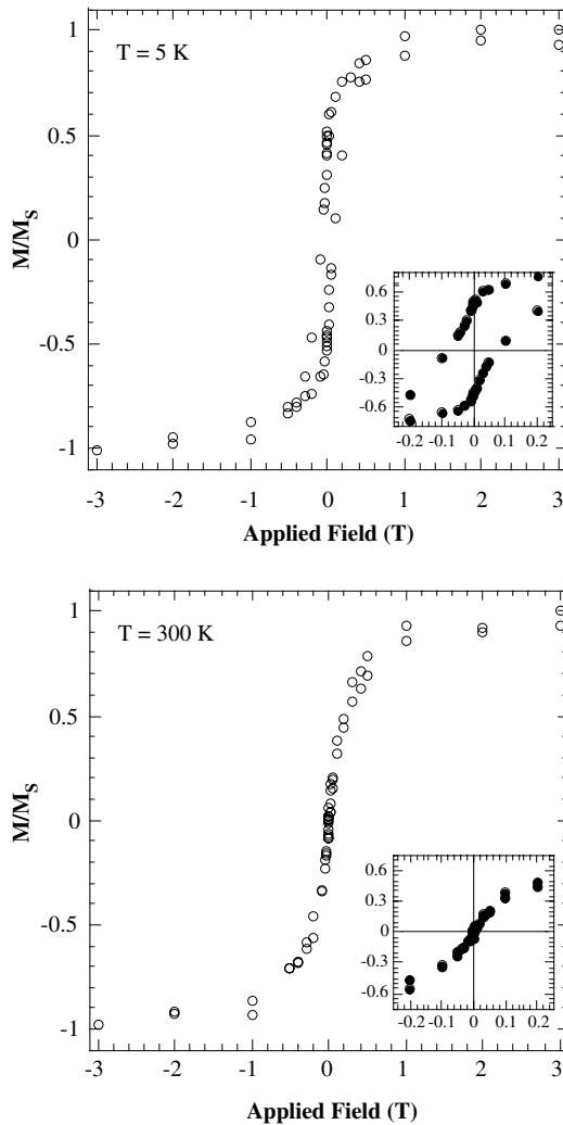
Fig. 3. Normalized magnetization loops at 5 K (top) and 300 K (bottom) for field applied parallel to the plane of a ZnO sample implanted with 5 at.% Co.
