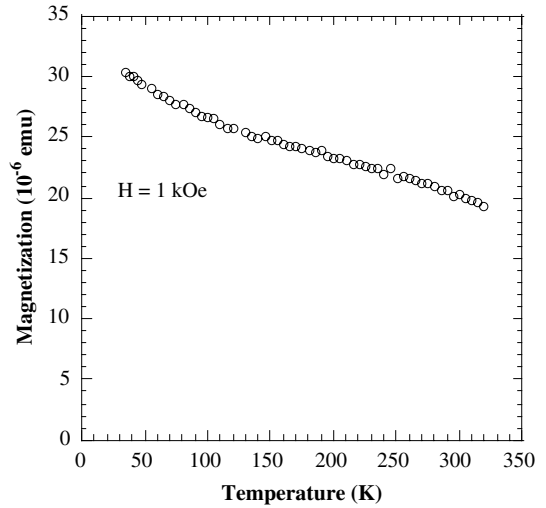
Fig. 2. Temperature dependence of magnetization at a field of 1000 G for a ZnO sample implanted with 3 at.% Co.
