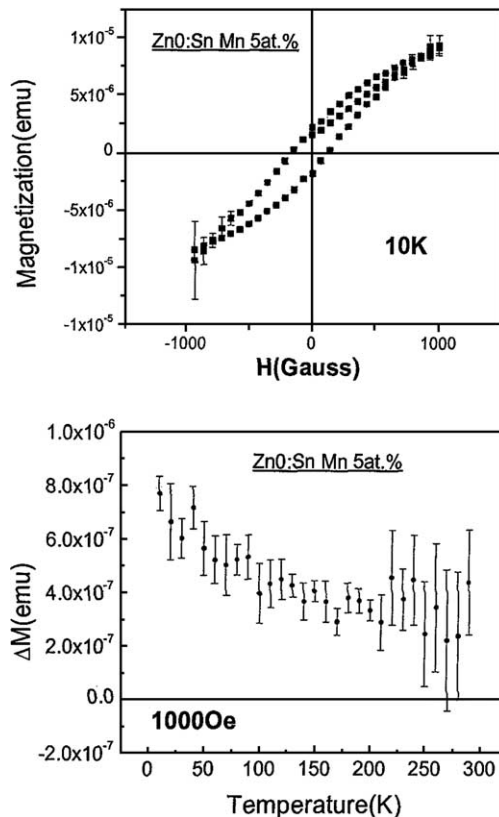
Fig. 6. Magnetization loop at 10 K for field applied perpendicular to the phase of a ZnO sample implanted with 5 at.% Mn (top) and temperature dependence of the difference of field-cooled and zero field-cooled magnetization at a field of 1000 Oe (bottom).
