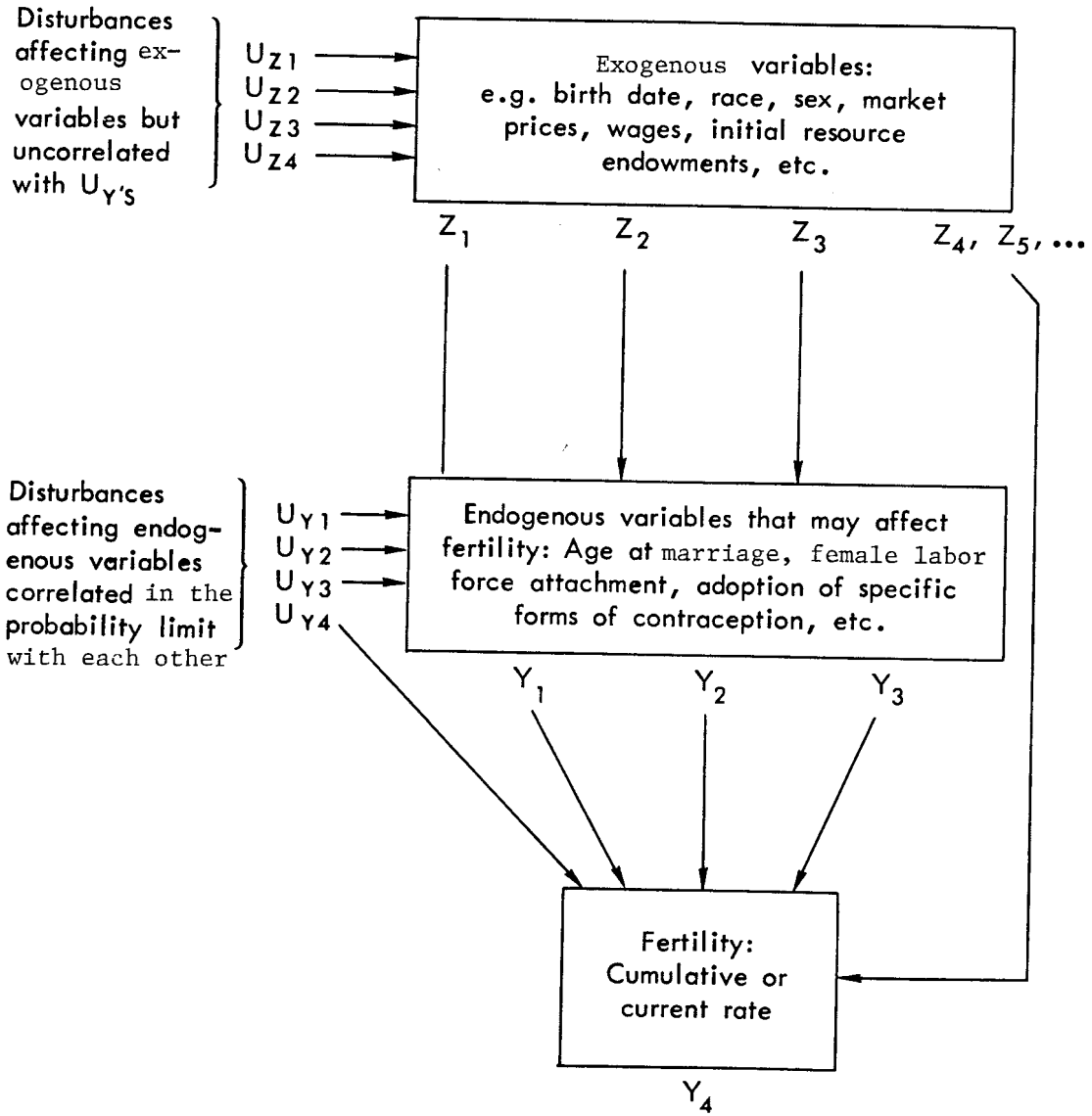
Fig.1—General causal framework for statistical analysis of factors affecting fertility
