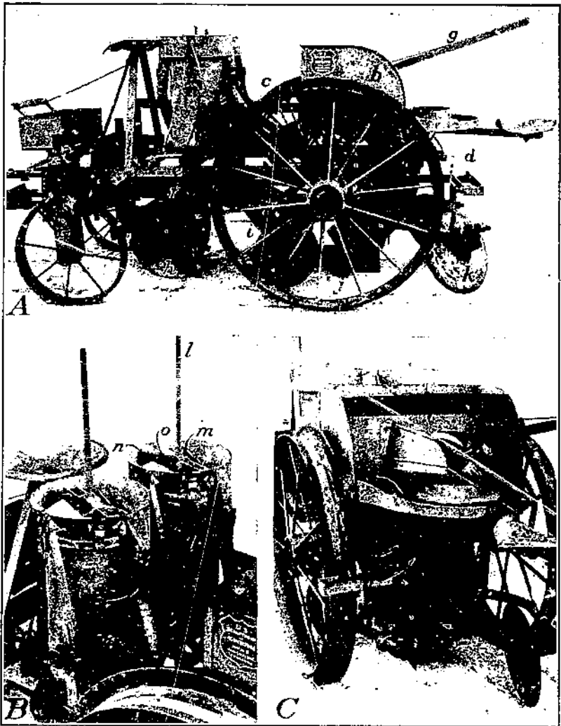
FIGURE 8.—A special combined potato planter and fertilizer distributor used in the fertilizer-placement studies with potatoes. A, General design of the machine: a , Fertilizer hopper; b , standard potato-planting mechanism; c , 2-inch flange on the drive wheel; d , wheel scraper; e , interchangeable sprockets in the fertilizer-hopper drive system; f , subframe to which all soil-working tools were attached; g , lever for adjusting the subframe vertically and controlling the driving mechanisms; h , pair of single-disk furrow openers for placing the fertilizer in a band at each side of the row; i , auxiliary bedding disks for returning disturbed soil to the row ahead of the seed shoe; j , seed shoe; k , seed-covering or bedding disks. B, Fertilizer hoppers of the rotating-cylinder top-delivery type: l , Plunger lifting screw; m , split-nut for releasing the lifting screw; n , fertilizer-discharge opening; o , fertilizer-delivery blade; p , fertilizer-delivery tube; q , rotating cylinder. C, Potato-planting mechanism of the cell-conveyor type with a seed-spacing attachment: r , Seed-elevating wheel; s , feed wheel on which the operator corrects the feed; t , seed-spacing attachment synchronized with the feed wheel; u , cam for operating the fertilizer hill-placement device; v , rod to transmit cam action to fertilizer valves.
