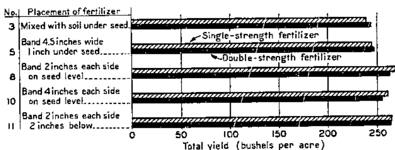
FIGURE 19.—Average total yield of potatoes for both single-strength and double-strength fertilizers in the following experiments—Maine, 1932-34; New Jersey, 1931-33; Virginia, 1932-34 and Michigan (Greenville), 1931. The numbers of the different fertilizer placements are given for convenience in referring to the corresponding sketches in figure 5.
