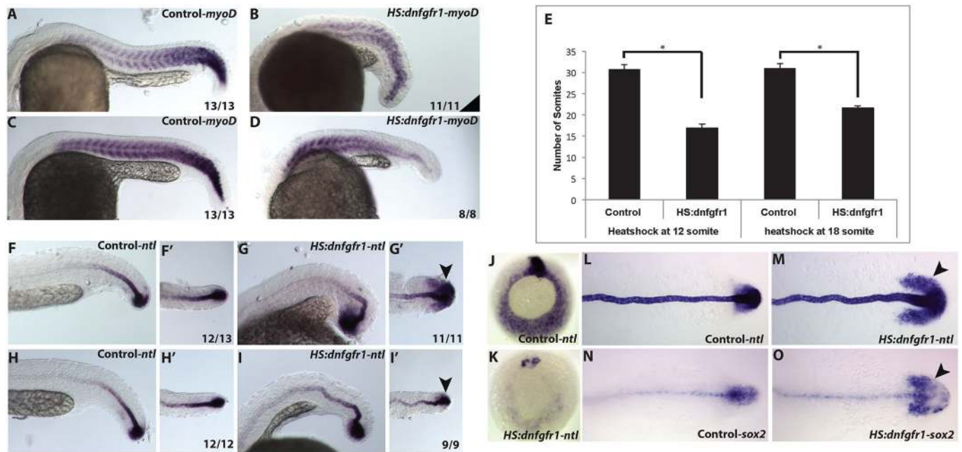
Fig. 1. FGF is required for post-gastrula mesoderm induction and repression of the NMP state. (A-E) Zebrafish embryos from an HS:dnfgr1 hemizygous outcross were heat shocked at the 12- or 18-somite stage and analyzed for myoD expression at 24 hpf. Wild-type siblings exhibit ~31 somites (A,C,E), whereas HS:dnfgr1 embryos heat shocked at 12 somites have 16 somites and those heat shocked at 18 somites have 22 somites (B,D,E). The number of embryos showing the illustrated phenotype among the total number examined is indicated. Error bars indicate s.d. * P < 0.001 (using unpaired t -test). (F-I') Expression of ntla (arrowheads) indicates that there is no posterior loss of notochord after FGF inhibition at the 12- or 18-somite stage. (J,K) Embryos heat shocked at 50% epiboly (just at the start of gastrulation) and fixed 3 h after heat shock show a near complete loss of ntla expression. (L,M) Embryos heat shocked at the 8-somite stage and fixed 3 h later exhibit an expansion of ntla into lateral and anterior domains (arrowhead). (N,O) Inhibition of FGF signaling at the 8-somite stage also leads to an expansion of sox2 3 h after the heat shock. (A-D,F,G,H,I) Lateral view, anterior left; (F',G',H',I',L-O) dorsal view, anterior left; (J,K) vegetal view, dorsal top.
