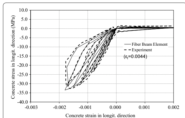
Fig. 8 Panel CVE3-1 concrete stress–strain behavior comparison with fiber beam element, and experiment (Mansour 2001).
