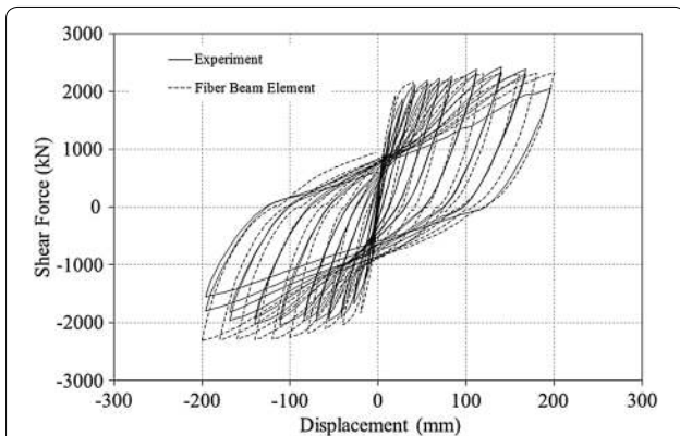
Fig. 13 Comparison of load–displacement behavior of specimen PI1 with fiber beam element, and experiment (Yeh and Mo 1999).
