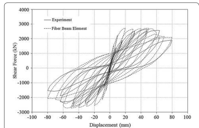
Fig. 14 Comparison of load–displacement behavior of specimen PI2 with fiber beam element, and experiment (Yeh and Mo 1999).
