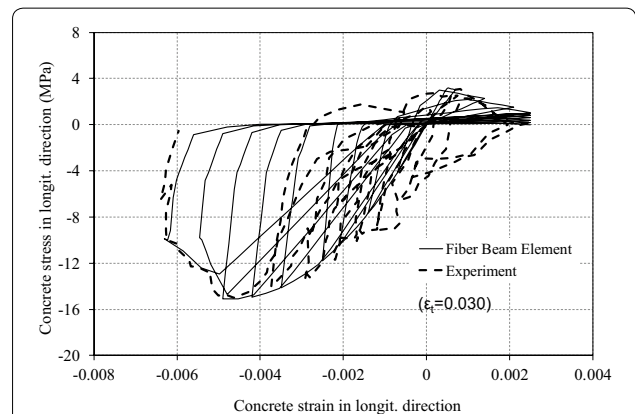
Fig. 10 Panel CVE3-3 concrete stress–strain behavior comparison with fiber beam element, and experiment (Mansour 2001).
