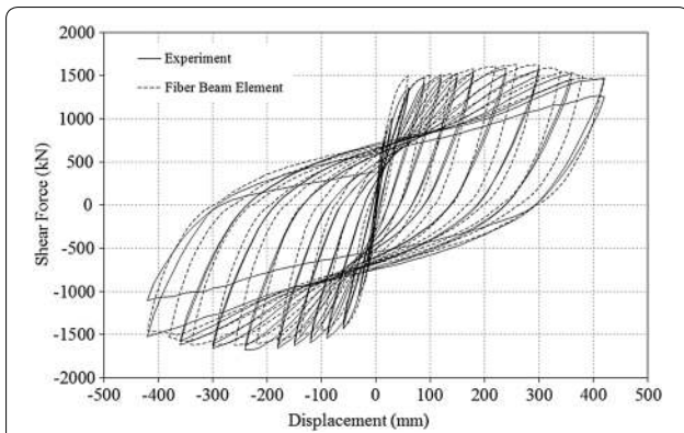
Fig. 12 Comparison of load–displacement behavior of specimen PS1 with fiber beam element, and experiment (Yeh and Mo 1999).
