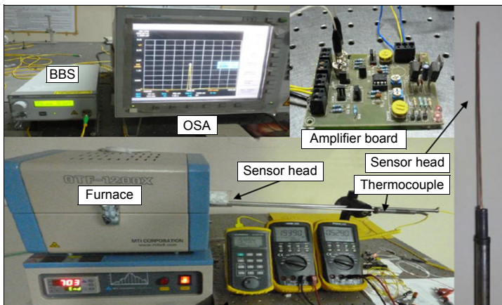
Fig. 4. Photographs of the experimental setup.
