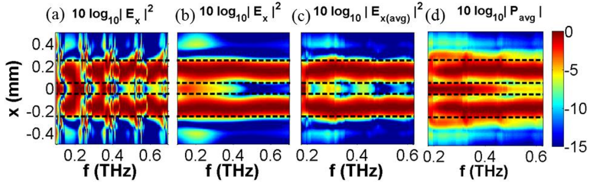
Fig. 13 (a) Simulated field intensity of two 200 \mu\text{m} diameter apertures with 100 \mu\text{m} inner-edge separation as a function of position and frequency. Same as (a) after (b) convolving field with the sinc function, (c) field average, and (d) power average over a full spectral range [72].
