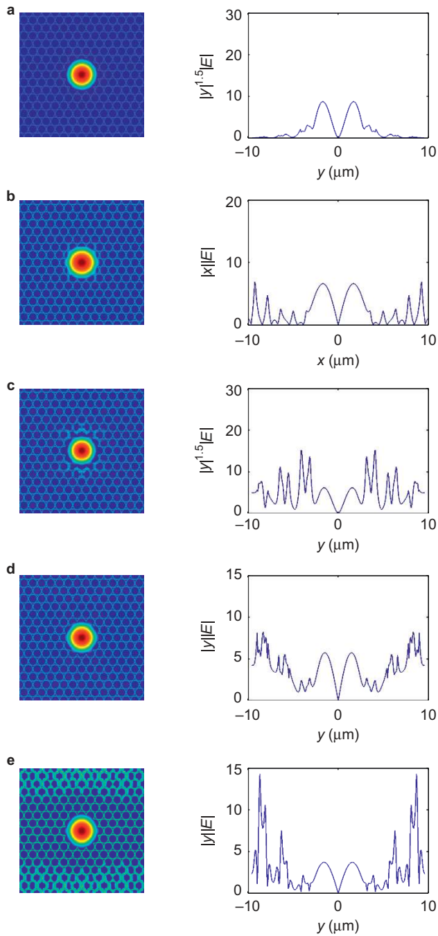
Figure 3 Guided modes in a triangular lattice photonic crystal fiber of germania glass. The fiber structure is shown in Figure 1a, where a=2.21\ \mu\text{m} , r_a=0.47a , R=1.9a , and \epsilon_r=1.59^2 . The modes were numerically calculated using the PWE method. The light-blue circles in the dark blue background give the positions of the hole-glass interfaces. (a–e) correspond to the red diamonds labeled 3a–3e in Figure 2b: (a) a gap mode ( \omega a/2\pi c=1.432 ), (b) a mode at a frequency between the photonic band gap and the lower edge of the Dirac spectrum ( \omega a/2\pi c=1.601 ), (c) the Dirac mode ( \omega a/2\pi c=1.689 ), (d) a mode in the Dirac spectrum ( \omega a/2\pi c=1.761 ), and (e) a mode at a frequency higher than the upper edge of the Dirac spectrum ( \omega a/2\pi c=1.950 ). The electric-field pattern |E| is shown on the left, and the product r^{3/2}|E| or r|E| on the x - or y -axis is shown on the right.
