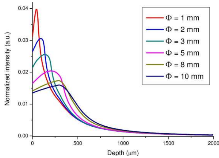
Fig. 8. The 785-nm illumination light distribution along the tissue depth using the Raman probe designs with different diameters of the ball lens ( \Phi = 1, 2, 3, 5, 8 and 10 mm).
