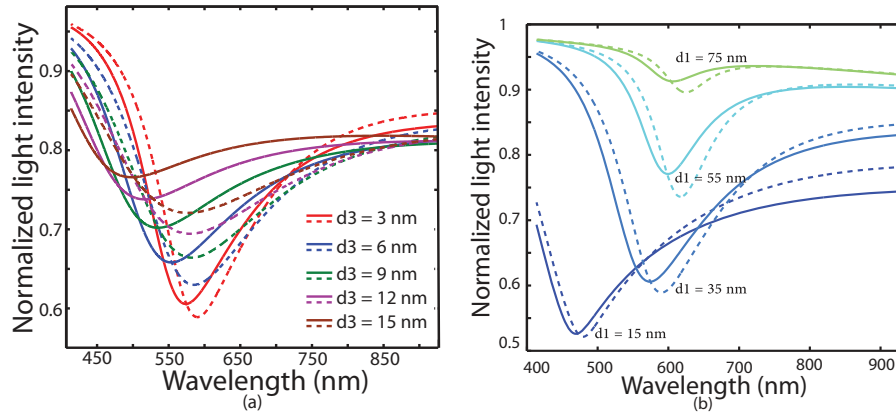
Fig. 6. Normalized light intensity as a function of the wavelength for (a) different thickness ( d_3 ) of Pd and (b) different thickness ( d_1 ) of Ag. The transducer is a multilayer made of d_1 nm Ag / d_2 nm SiO_2 / d_3 nm Pd. (NA = 0.22, core radius = 100 \mu m, L = 1 cm). The lines and dash lines represent the metallic and hydrogenated state, respectively.
