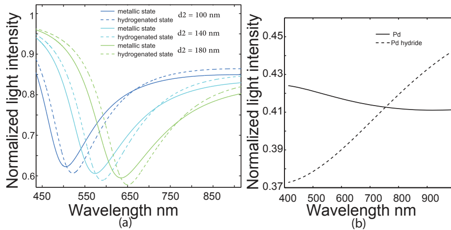
Fig. 2. (a) The transmitted light intensity as a function of the wavelength for different thickness of \text{SiO}_2 . The transducer is a multilayer composed of 35 nm Ag / d_2 nm \text{SiO}_2 / 3 nm Pd. (NA = 0.22, core radius = 100 \mu\text{m} , L = 1 cm). (b) The transmitted light intensity as a function of the wavelength, where the transducer is a 10 nm Pd layer (NA = 0.22, core radius = 100 \mu\text{m} , L = 2 cm)
