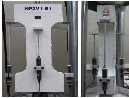
Fig. 2. Test set-up.
