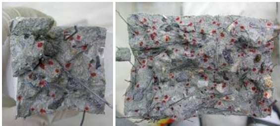
(a) NF1V3-S5 (b) NF3V3 Fig. 4. Counting the number of fibers.
