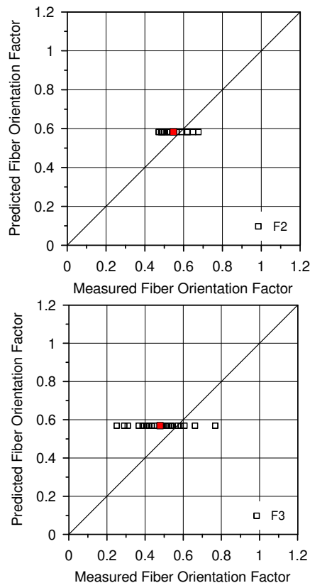
Fig. 7. Comparison of the prediction and the test results on fiber orientation factor.
