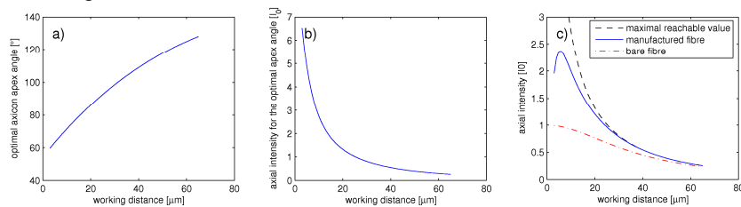
Fig. 2. (a). Optimal angle of the axicon tip as a function of the working distance (b) the maximum beam intensity obtained at each working distance using the optimal fibre. I_0 is the on-axis intensity of the fibre mode (c) comparison of the on-axis intensity of the fabricated fibre with the maximal achievable intensity for the optimal fibre (Fig. 2(b)) and the bare-tipped fibre.
