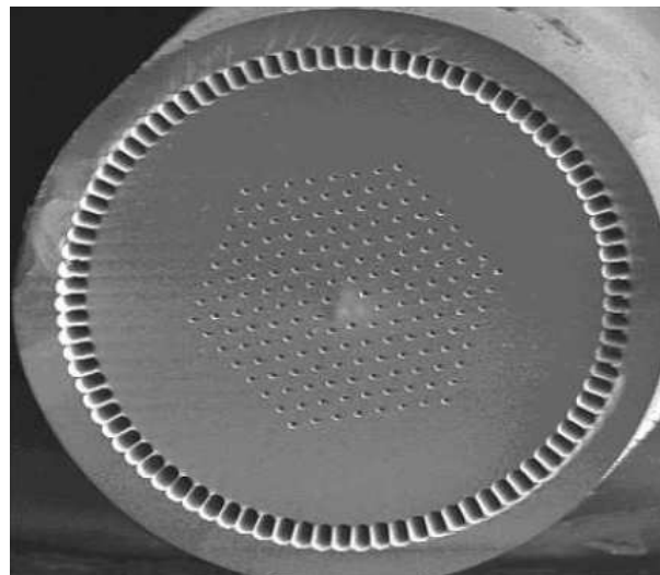
Fig. 6. Cross-section of photonic fibre
