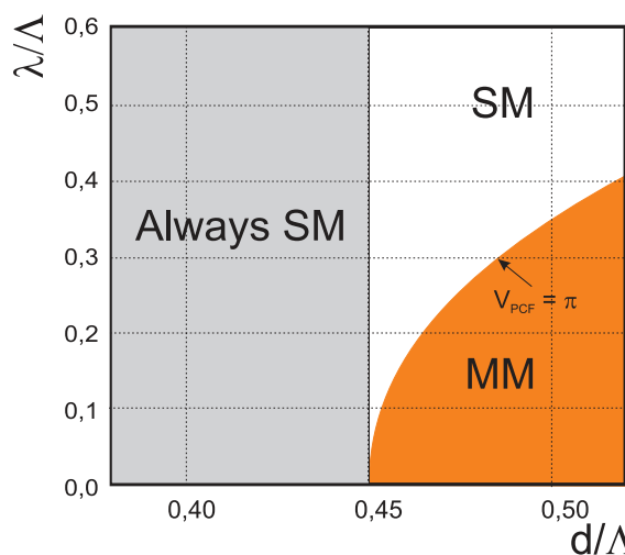
Fig. 7. Classification of photonic fibre based on modality of structures. In the photonic fibre set-up for the relation of air channel diameter d to the period of structure \Lambda lower from 0.45 the fibre is always SM
