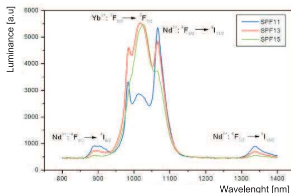
Fig. 10. Luminescence spectra of doped glass with Nd 3+ /Yb 3+ (SPF11, SPF13, SPF15) \lambda_p = 808 nm
