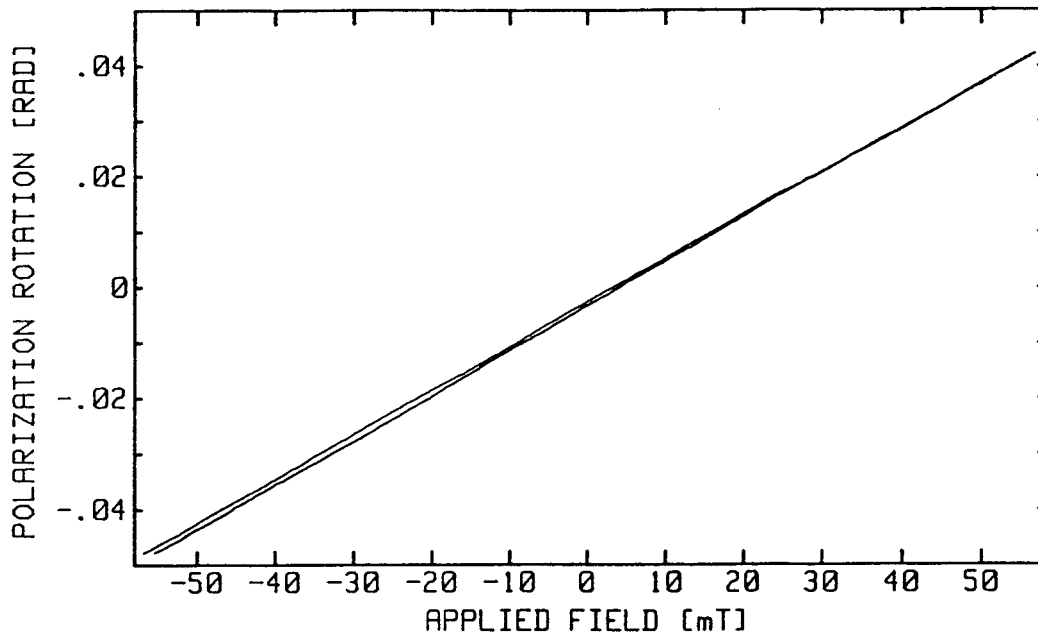
Fig. 5 Polarization rotation in 0.3 \times 1.4 \times 1.4 mm YIG slice. Measured parallel with (1.1.1) direction, perpendicular to slice with 300 \mu\text{m} diameter light beam
