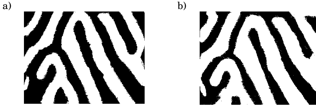
Fig. 18. Domain patterns in 0.3 mm slice of pure YIG. a) with no external field applied. b) with a magnetic field applied perpendicularly to the plane of the sample.
