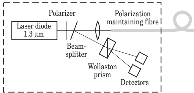
Fig. 32. Optoelectronic unit for one-fibre sensing system.
