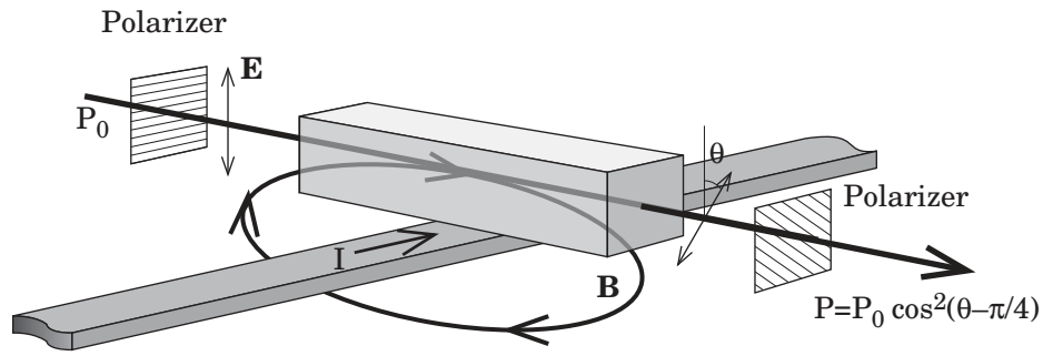
Fig. 7. The simplest form of an optical current sensor utilizing the Faraday effect.
