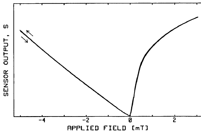
Fig. 14. Output signal S versus B_{\text{meas}} with a sensor according to fig 13 with a B_{\text{bias}} of 3 mT.
