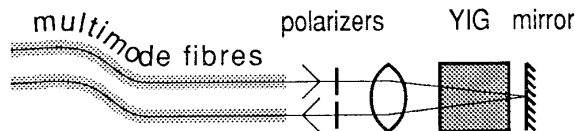
Fig. 1b. Principle outline of the reflection type magnetic field sensor
