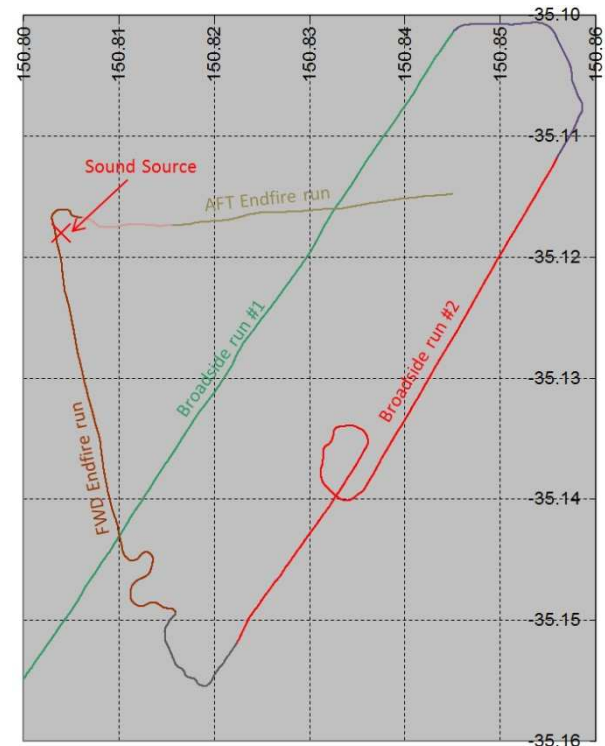
Figure 5. FOTA travel during its performance assessment
