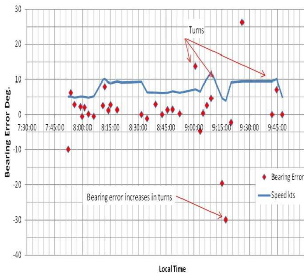
Figure 6. Bearing errors during performance assessment
