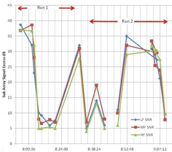
Figure 7. Signal excess during broadside runs
