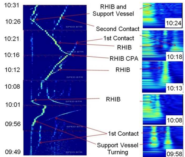
Figure 9. RHIB tracking summary
