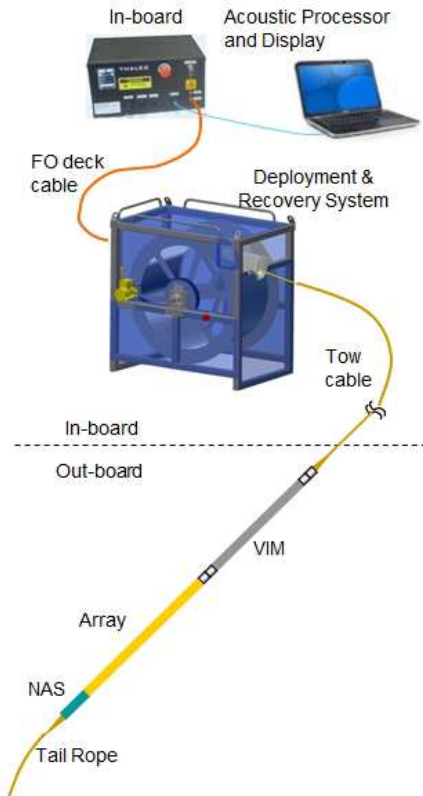
Figure 1. FOTA Demonstrator Sections
