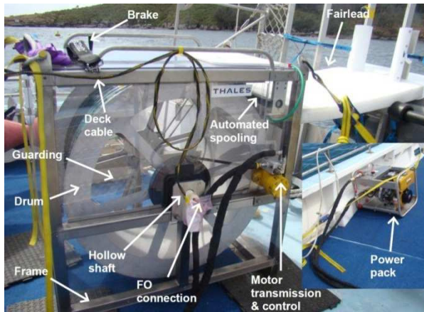
Figure 3. FOTA Deployment & Recovery system
