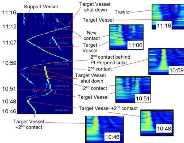
Figure 11. Diver Support Vessel tracking summary
