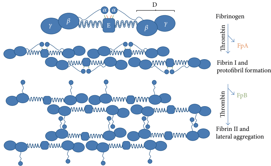
FIGURE 1: Schematic representation of the fibrin aggregation process. Fibrinogen is composed of two sets of A\alpha -, B\beta -, and \gamma chains. Each \alpha -chain is connected with E-region through fibrinopeptide A (FPA, orange) and fibrinopeptide B (FPB, green). The D-region is linked with E-region through a coiled segment. Thrombin-mediated cleavage of FPA induces the formation of two-stranded protofibril. Subsequent cleavage of FPB releases \alpha -chain from E-region and contributes to the lateral aggregation of two-stranded protofibrils and fibrin formation [24].
